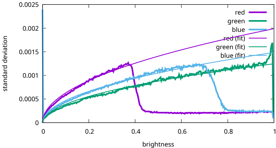
Noise levels - Sony, ILCE-7M3, 50 ISO (7M30954)
