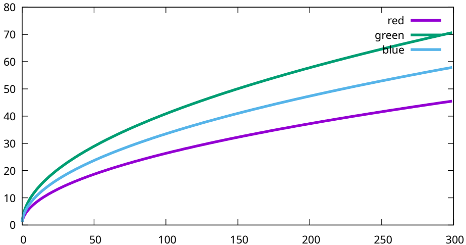
Conversion curves - Sony, ILCE-7M3, 160000 ISO (7M30989)
