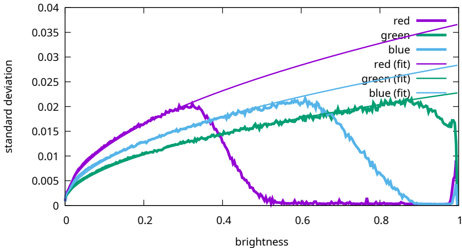
Noise levels - Sony, ILCE-7M3, 102400 ISO (7M30986)
