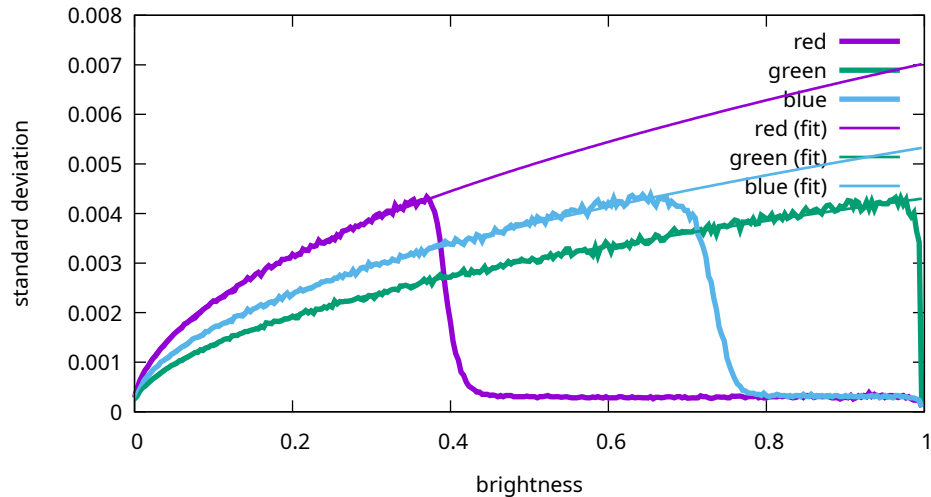
Noise levels - Sony, ILCE-7M3, 2000 ISO (7M30970)
