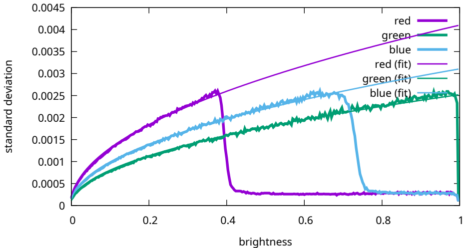
Noise levels - Sony, ILCE-7M3, 640 ISO (7M30965)
