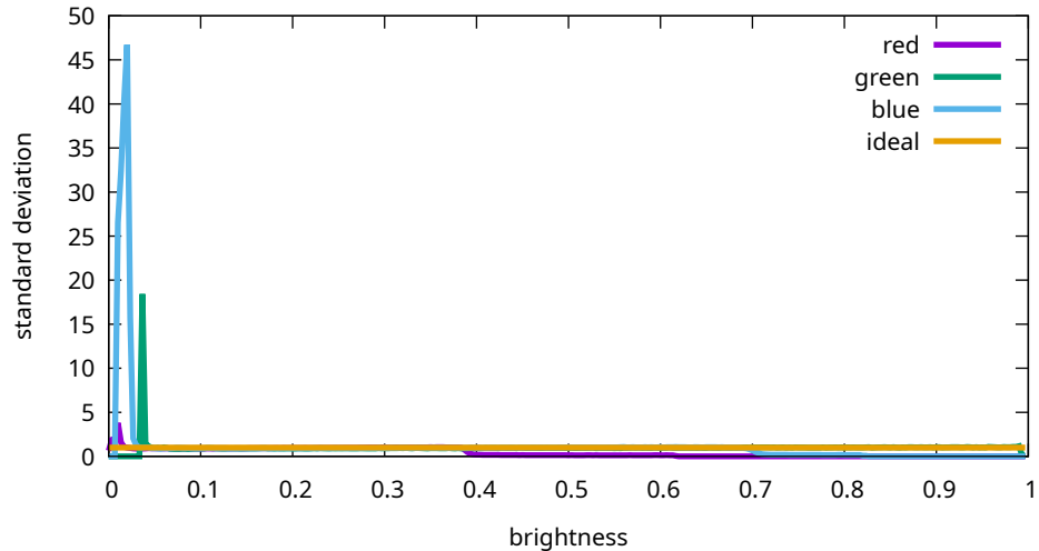
Flat noise levels - Sony, ILCE-7M3, 125 ISO (7M30958)
