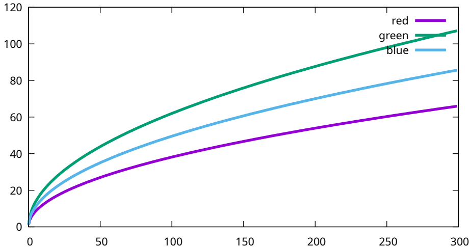
Conversion curves - Sony, ILCE-7M3, 40000 ISO (7M30983)
