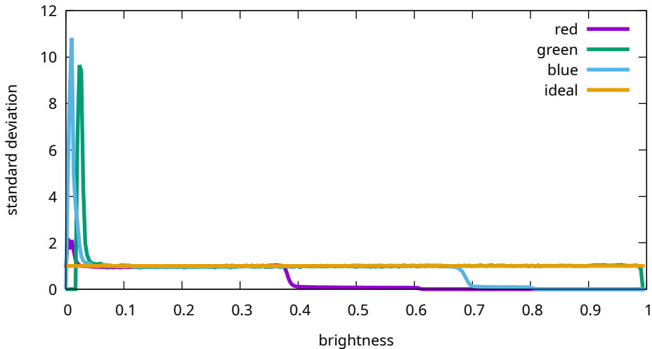
Flat noise levels - Sony, ILCE-7M3, 800 ISO ( 7 M30966)
