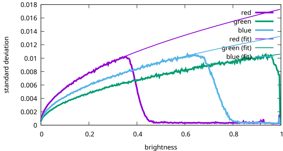
Noise levels - Sony, ILCE-7M3, 12800 ISO (7M30978)
