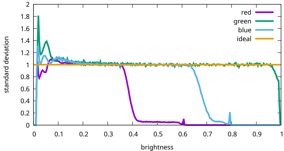
Flat noise levels - Sony, ILCE-7M3, 32000 ISO ( _7M30982 )
