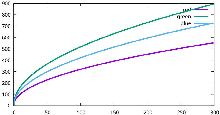
Conversion curves - Sony, ILCE-7M3, 500 ISO (7M30964)
