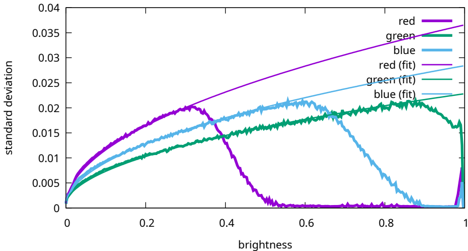
Noise levels - Sony, ILCE-7M3, 102400 ISO (7M30987)
