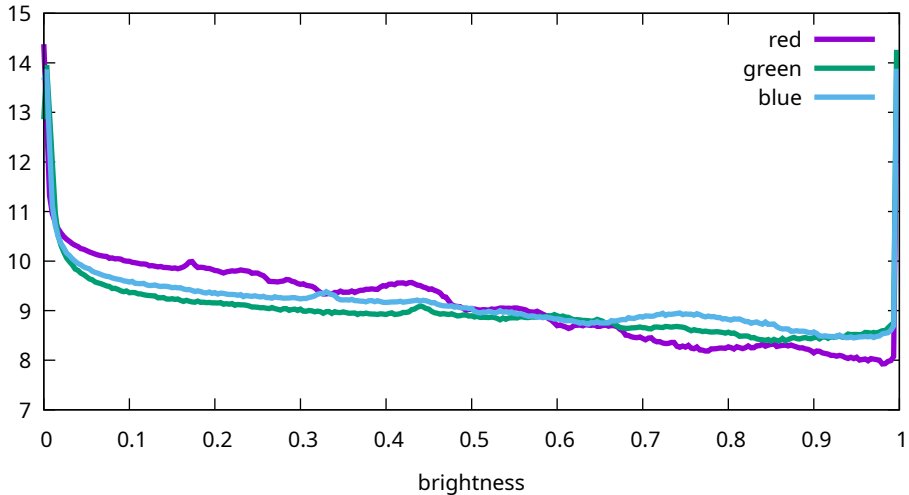
Flat histogram - Sony, ILCE-7M3, 160 ISO (7M30959)
