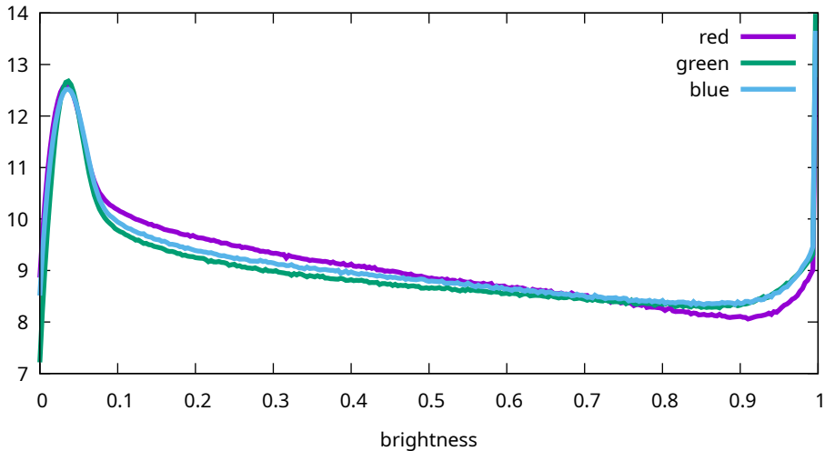
Flat histogram - Sony, ILCE-7M3, 204800 ISO (7M30990)
