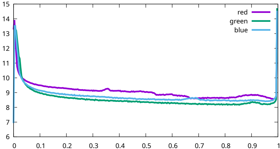
Histogram - Sony, ILCE-7M3, 64 ISO (7M30955)
