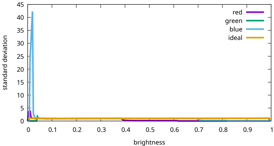
Flat noise levels - Sony, ILCE-7M3, 160 ISO (7M30959)
