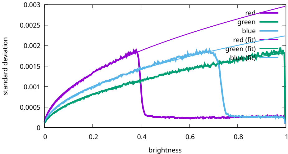
Noise levels - Sony, ILCE-7M3, 320 ISO (7M30962)
