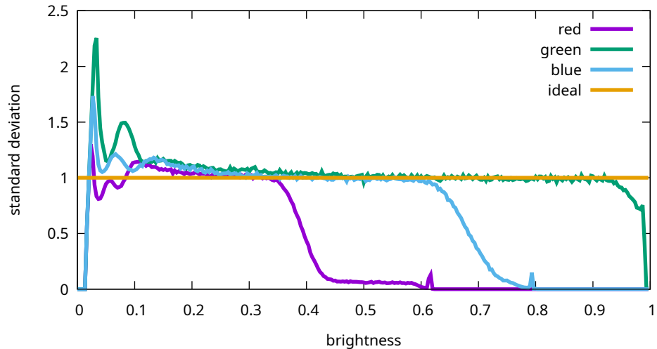
Flat noise levels - Sony, ILCE-7M3, 102400 ISO (7M30987)
