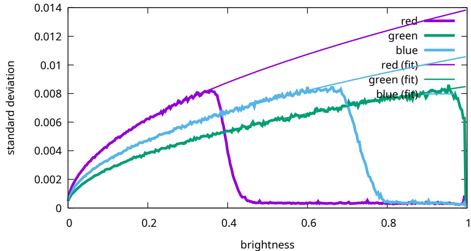
Noise levels - Sony, ILCE-7M3, 8000 ISO (7M30976)
