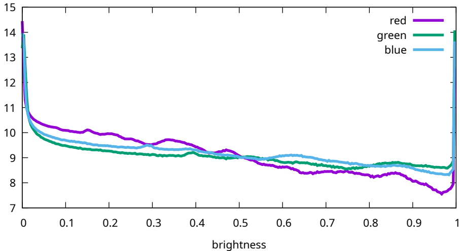
Flat histogram - Sony, ILCE-7M3, 1600 ISO (7M30969)
