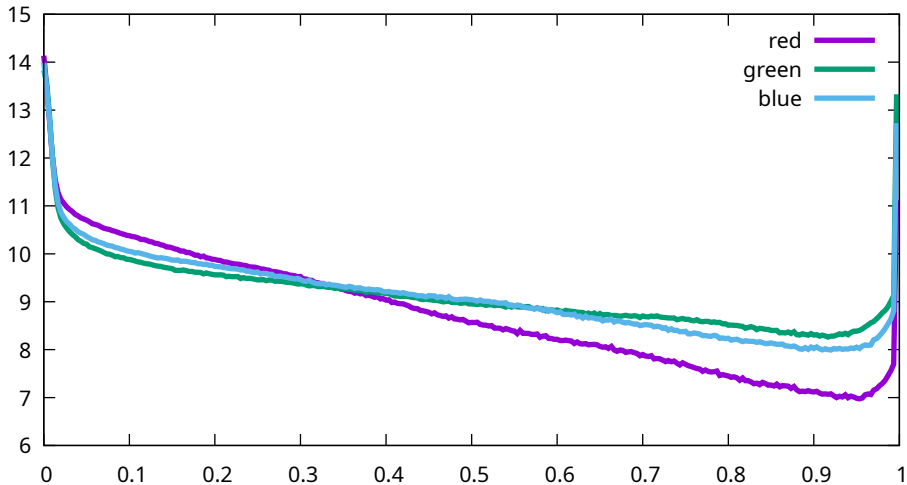
Histogram - Sony, ILCE-7M3, 64000 ISO (7M30985)
