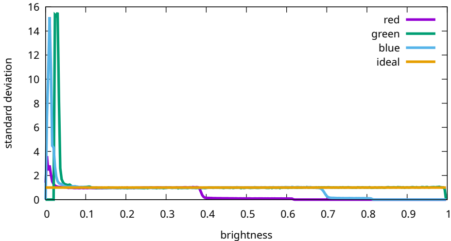
Flat noise levels - Sony, ILCE-7M3, 400 ISO ( 7M30963 )
