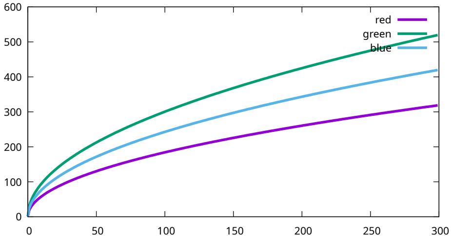
Conversion curves - Sony, ILCE-7M3, 1600 ISO (7M30969)
