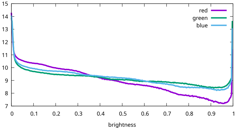
Flat histogram - Sony, ILCE-7M3, 25600 ISO (7M30981)
