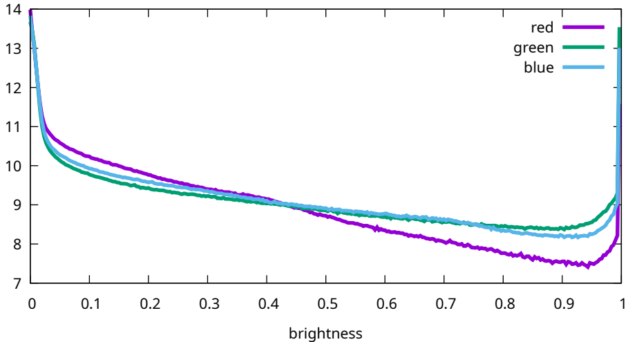
Flat histogram - Sony, ILCE-7M3, 102400 ISO (7M30987)
