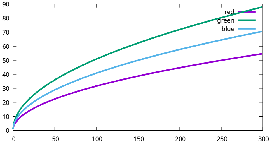
Conversion curves - Sony, ILCE-7M3, 102400 ISO (7M30986)
