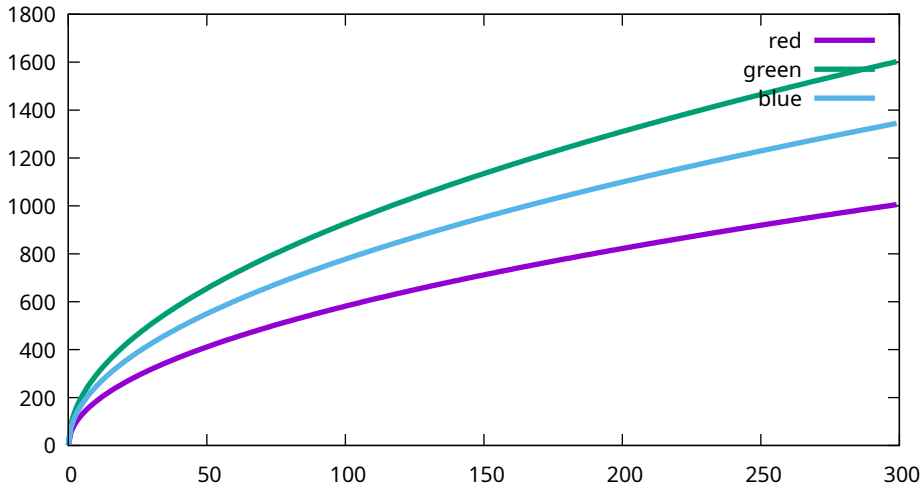
Conversion curves - Sony, ILCE-7M3, 50 ISO (7M30954)
