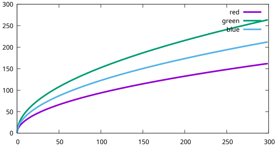
Conversion curves - Sony, ILCE-7M3, 6400 ISO (7M30975)
