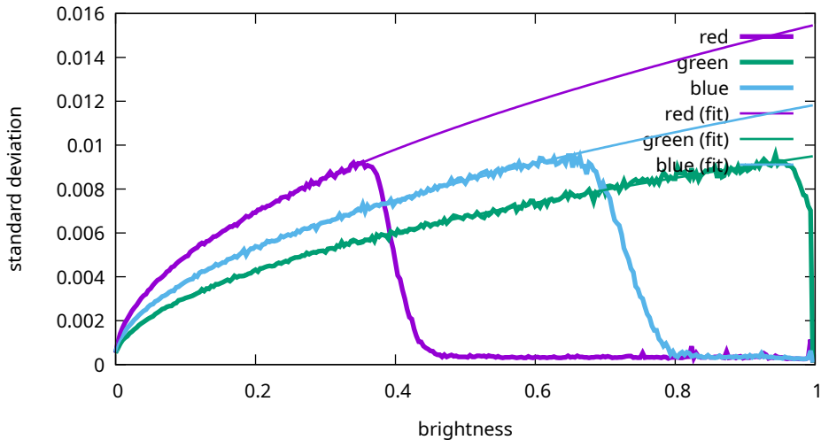
Noise levels - Sony, ILCE-7M3, 10000 ISO (7M30977)
