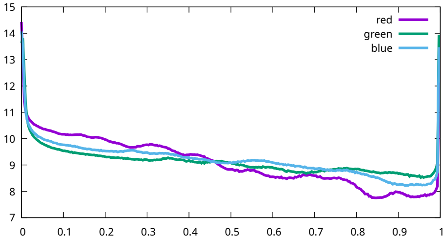
Histogram - Sony, ILCE-7M3, 6400 ISO (7M30975)
