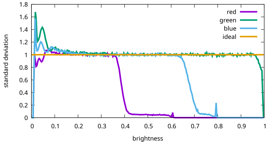
Flat noise levels - Sony, ILCE-7M3, 25600 ISO ( 7M30981 )
