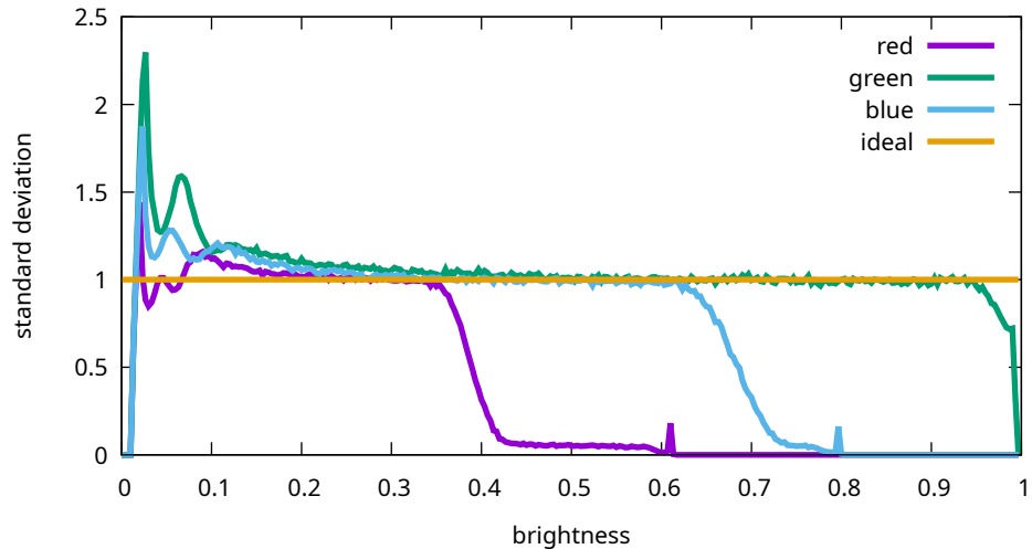
Flat noise levels - Sony, ILCE-7M3, 64000 ISO (7M30985)
