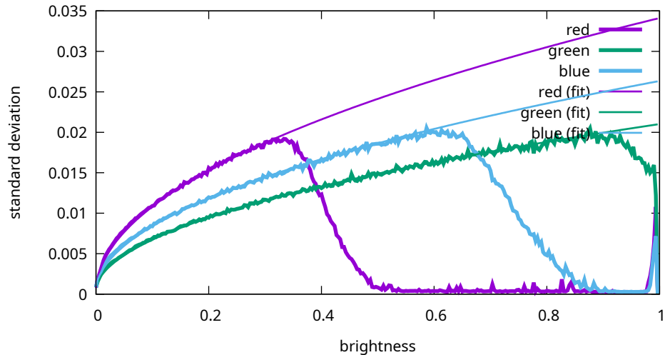
Noise levels - Sony, ILCE-7M3, 51200 ISO (7M30984)
