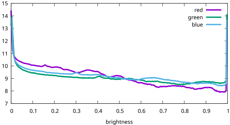
Flat histogram - Sony, ILCE-7M3, 800 ISO (7M30966)
