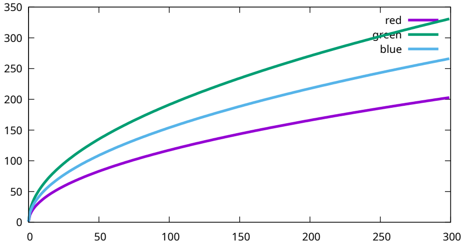
Conversion curves - Sony, ILCE-7M3, 4000 ISO (7M30973)
