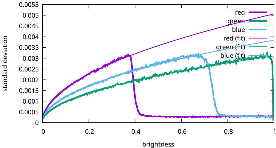
Noise levels - Sony, ILCE-7M3, 1000 ISO (7M30967)
