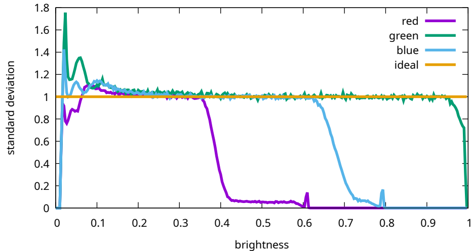
Flat noise levels - Sony, ILCE-7M3, 40000 ISO ( _7M30983 )
