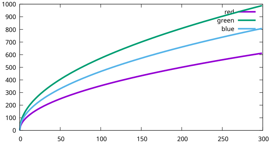
Conversion curves - Sony, ILCE-7M3, 400 ISO (7M30963)
