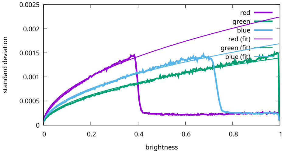
Noise levels - Sony, ILCE-7M3, 160 ISO (7M30959)
