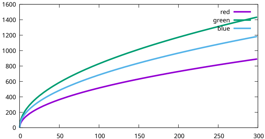
Conversion curves - Sony, ILCE-7M3, 160 ISO (7M30959)
