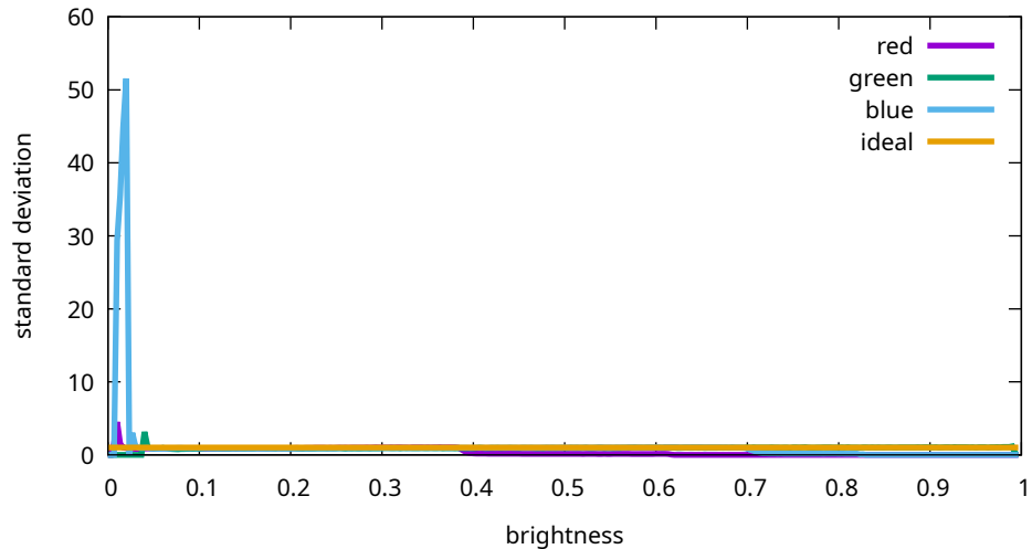
Flat noise levels - Sony, ILCE-7M3, 100 ISO (7M30957)
