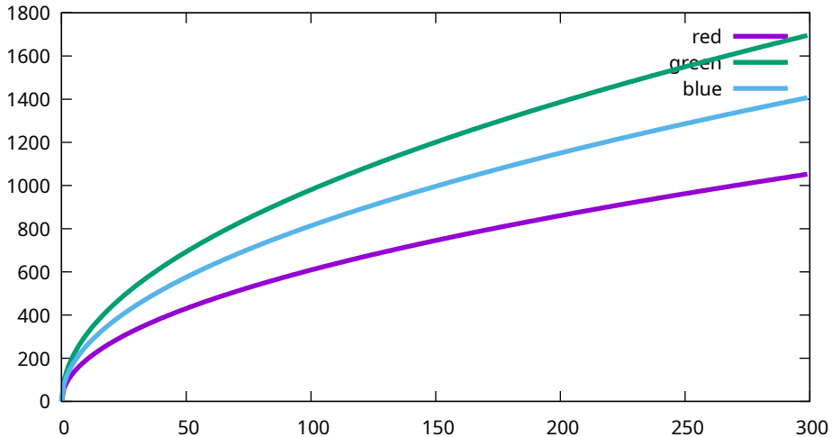
Conversion curves - Sony, ILCE-7M3, 100 ISO (7M30957)
