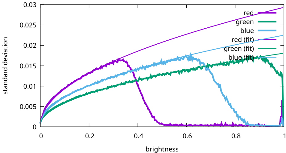
Noise levels - Sony, ILCE-7M3, 64000 ISO (7M30985)
