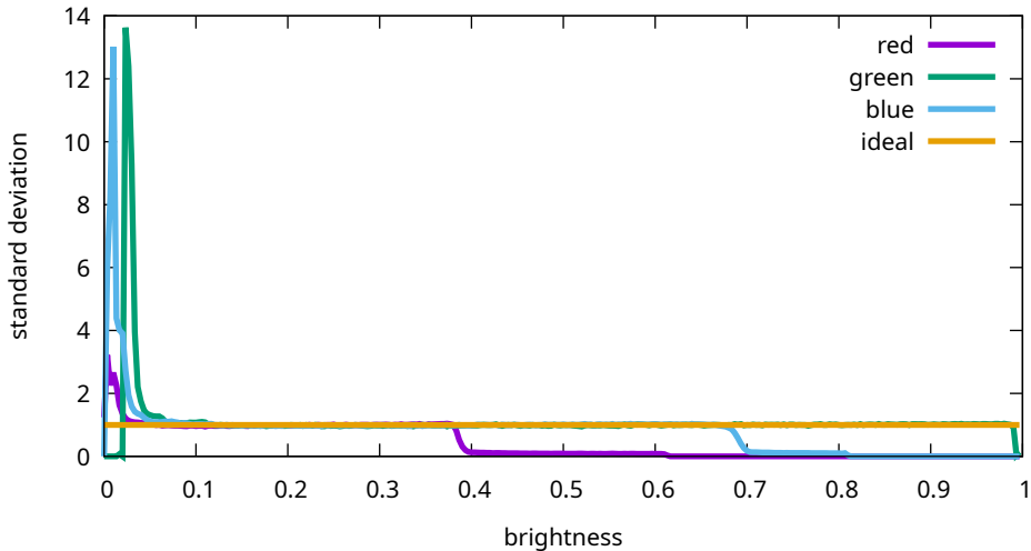
Flat noise levels - Sony, ILCE-7M3, 500 ISO ( 7 M30964)
