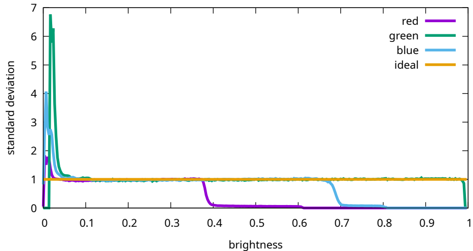
Flat noise levels - Sony, ILCE-7M3, 1250 ISO ( 7M30968 )
