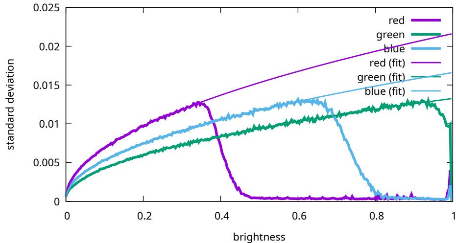
Noise levels - Sony, ILCE-7M3, 20000 ISO (7M30980)
