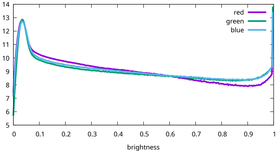
Flat histogram - Sony, ILCE-7M3, 160000 ISO (7M30989)
