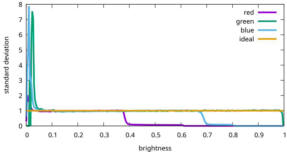
Flat noise levels - Sony, ILCE-7M3, 1000 ISO (7M30967)
