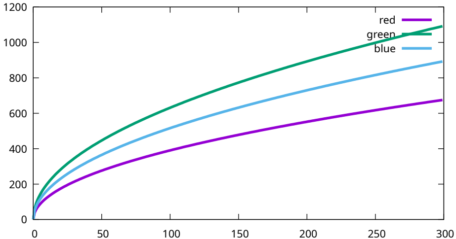
Conversion curves - Sony, ILCE-7M3, 320 ISO (7M30962)
