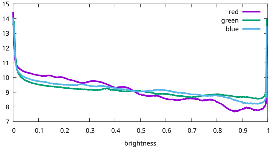
Flat histogram - Sony, ILCE-7M3, 5000 ISO (7M30974)
