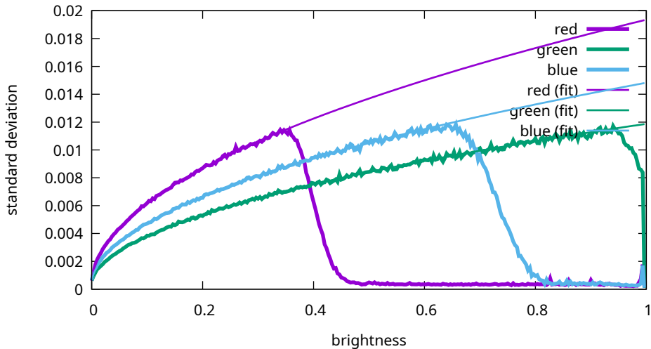
Noise levels - Sony, ILCE-7M3, 16000 ISO (7M30979)
