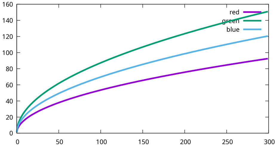
Conversion curves - Sony, ILCE-7M3, 20000 ISO ( 7 M30980)
