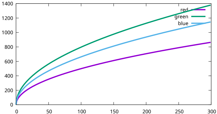
Conversion curves - Sony, ILCE-7M3, 80 ISO (7M30956)
