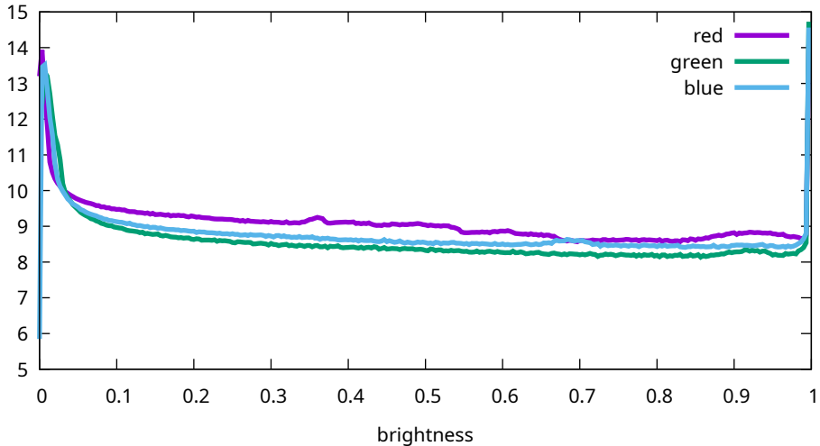
Flat histogram - Sony, ILCE-7M3, 50 ISO (7M30954)
