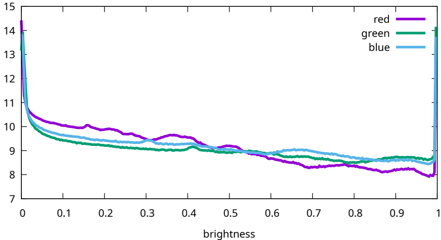
Flat histogram - Sony, ILCE-7M3, 640 ISO (7M30965)
