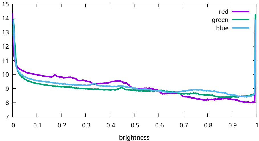
Flat histogram - Sony, ILCE-7M3, 125 ISO (7M30958)
