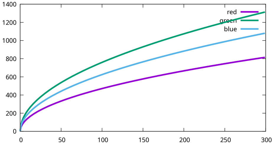
Conversion curves - Sony, ILCE-7M3, 200 ISO (7M30960)
