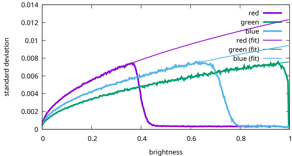
Noise levels - Sony, ILCE-7M3, 6400 ISO (7M30975)
