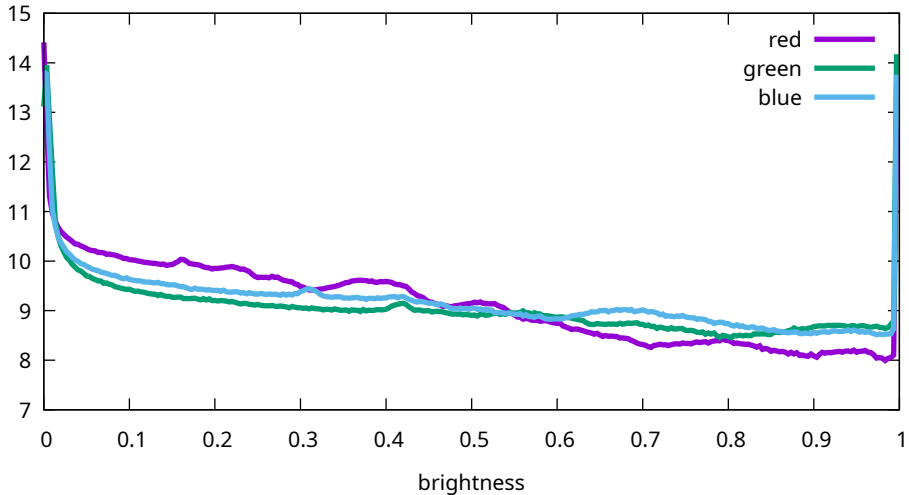
Flat histogram - Sony, ILCE-7M3, 500 ISO (7M30964)
