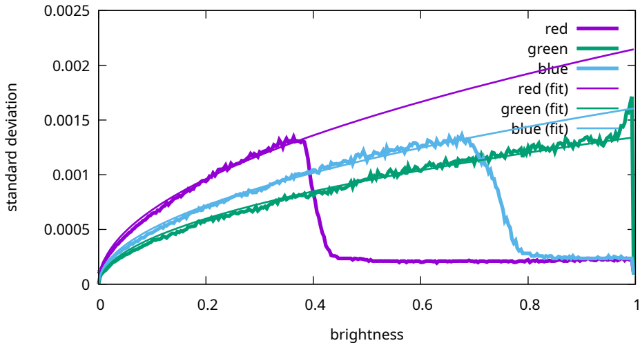
Noise levels - Sony, ILCE-7M3, 64 ISO (7M30955)
