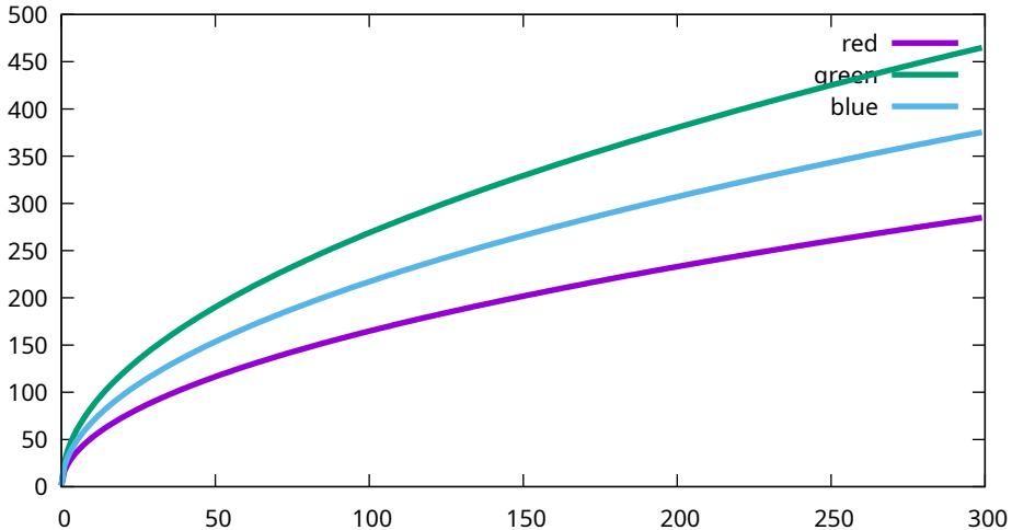
Conversion curves - Sony, ILCE-7M3, 2000 ISO (7M30970)
