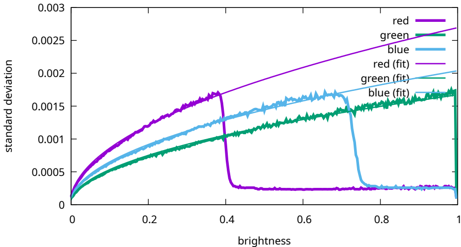
Noise levels - Sony, ILCE-7M3, 250 ISO (7M30961)
