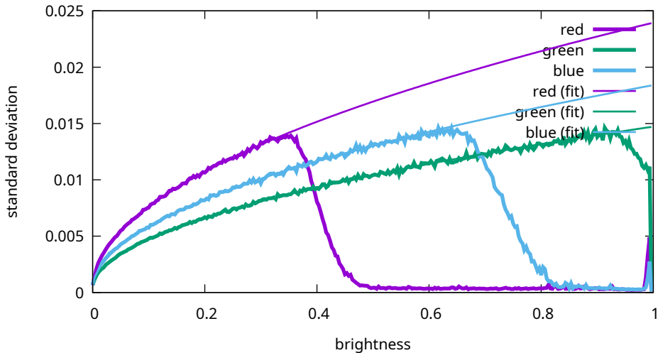
Noise levels - Sony, ILCE-7M3, 25600 ISO (7M30981)
