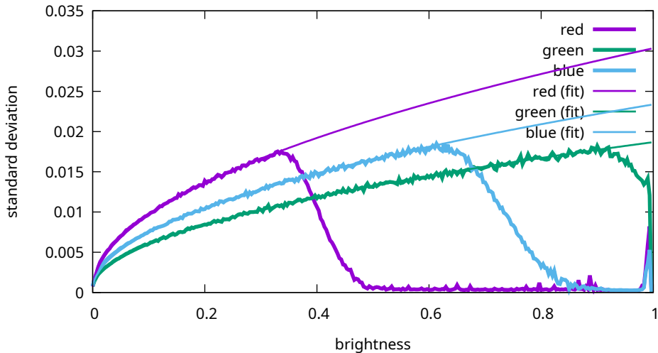
Noise levels - Sony, ILCE-7M3, 40000 ISO (7M30983)
