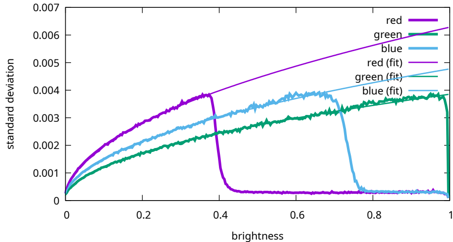
Noise levels - Sony, ILCE-7M3, 1600 ISO (7M30969)
