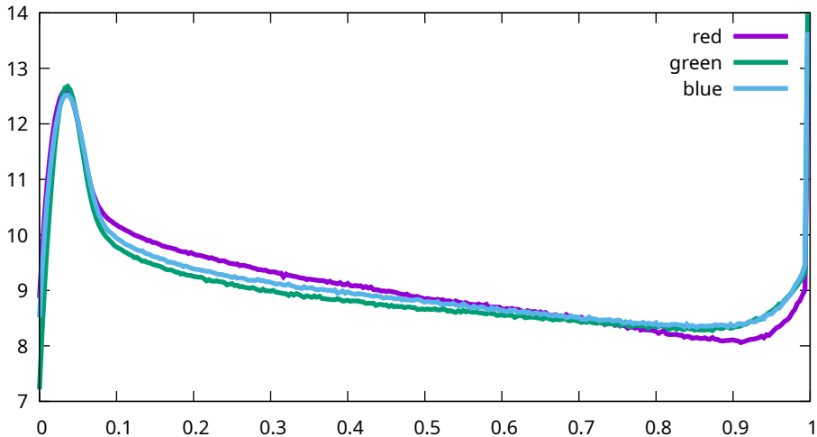
Histogram - Sony, ILCE-7M3, 204800 ISO (7M30990)
