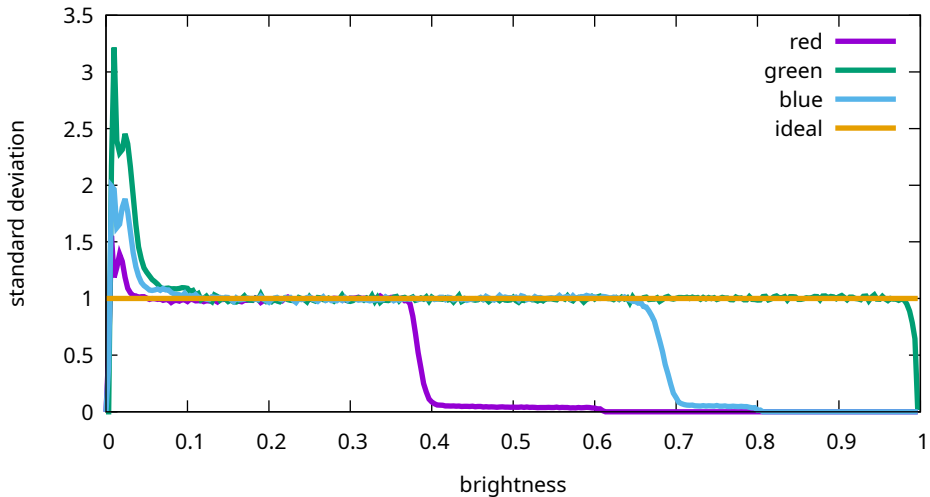
Flat noise levels - Sony, ILCE-7M3, 4000 ISO (7M30973)
