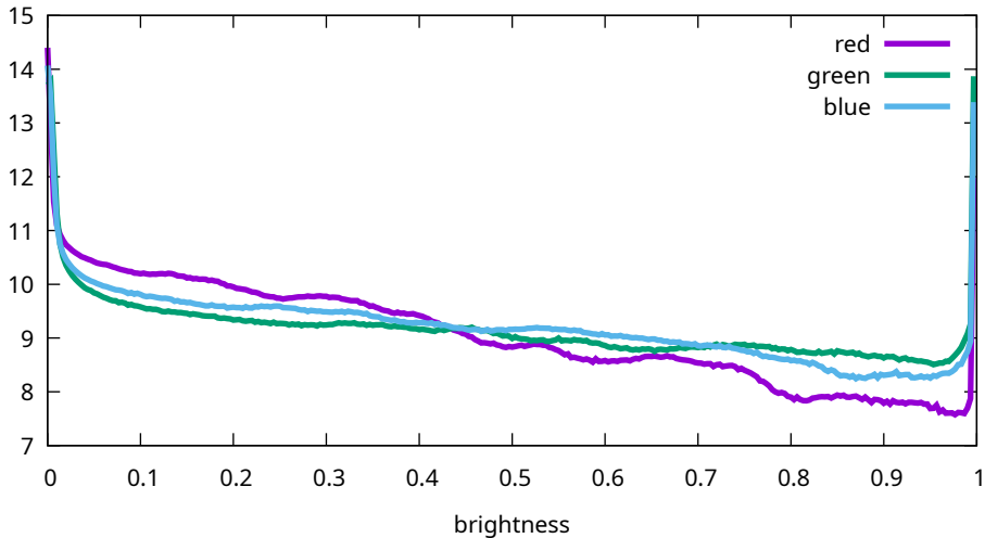
Flat histogram - Sony, ILCE-7M3, 10000 ISO (7M30977)
