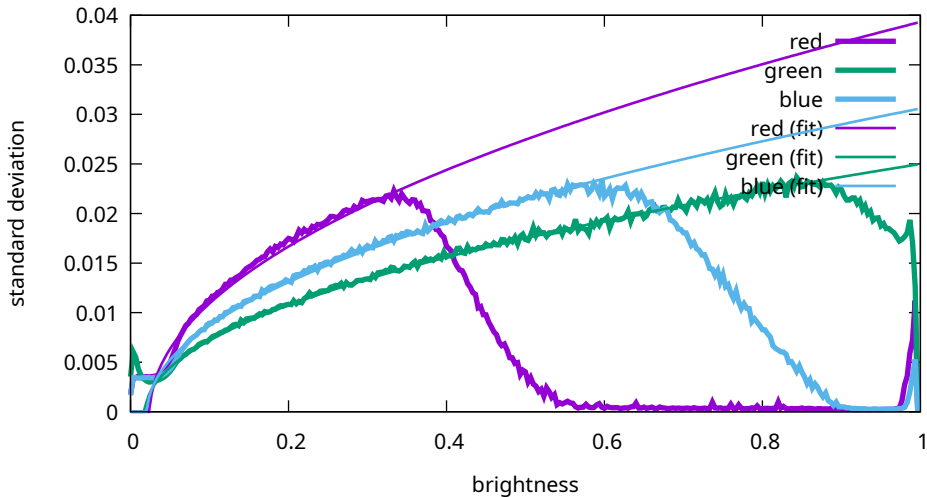
Noise levels - Sony, ILCE-7M3, 128000 ISO ( 7 M30988)
