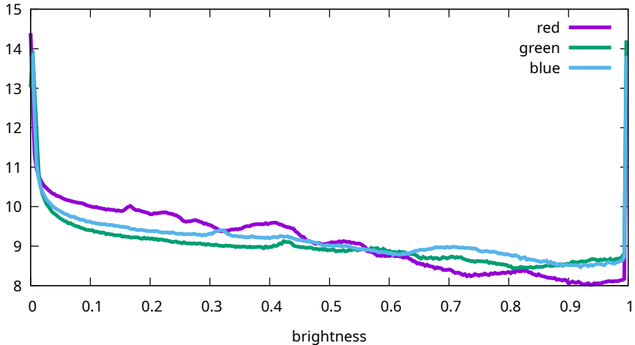
Flat histogram - Sony, ILCE-7M3, 320 ISO (7M30962)
