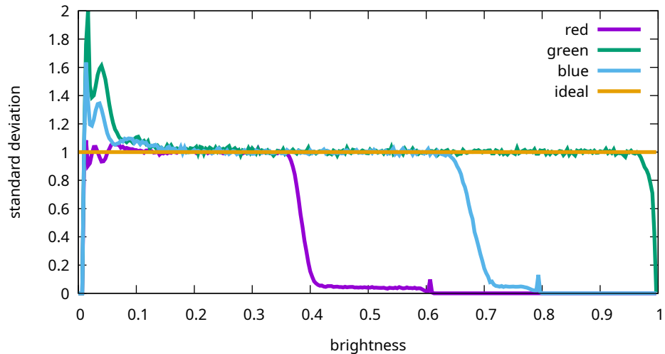
Flat noise levels - Sony, ILCE-7M3, 16000 ISO ( 7M30979 )
