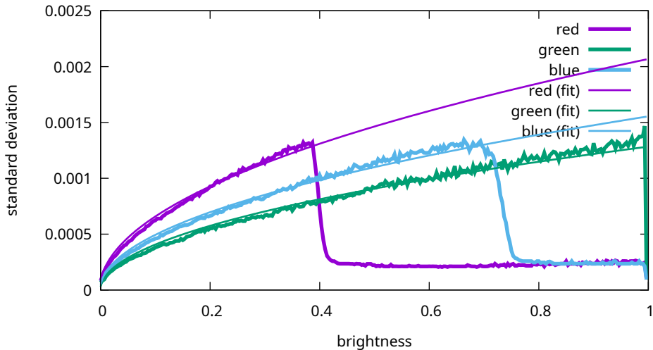
Noise levels - Sony, ILCE-7M3, 125 ISO (7M30958)
