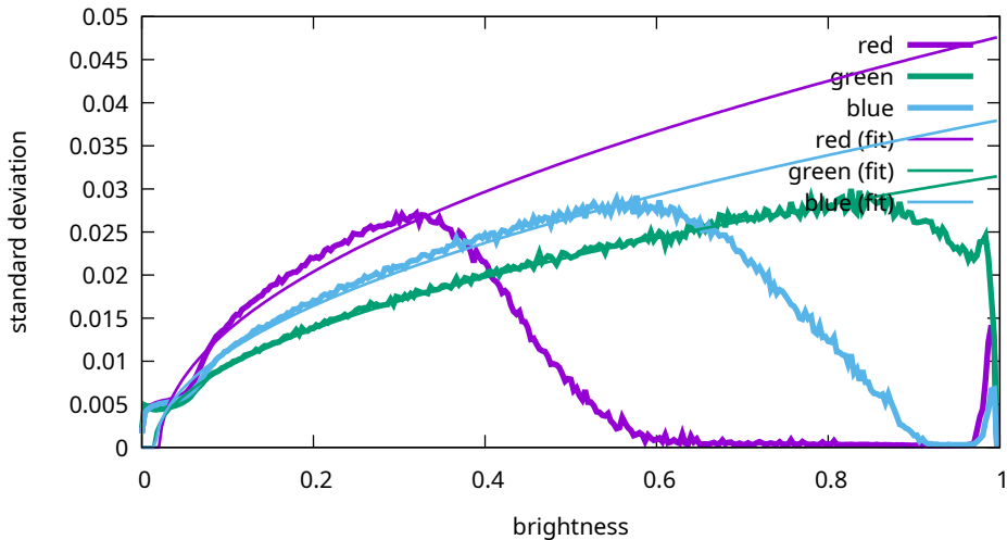
Noise levels - Sony, ILCE-7M3, 204800 ISO ( \gamma M30990)
