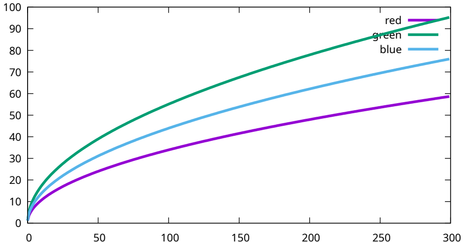
Conversion curves - Sony, ILCE-7M3, 51200 ISO (7M30984)
