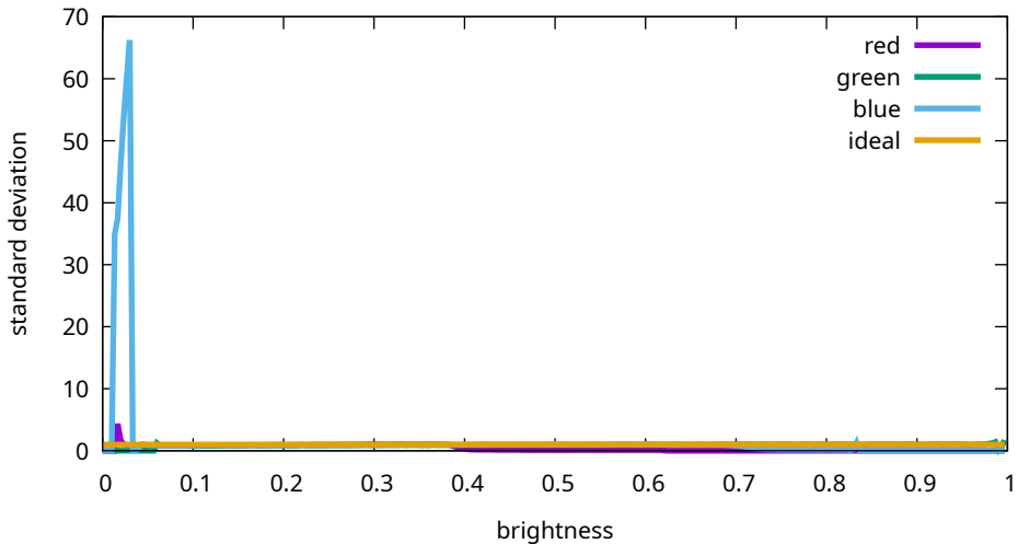
Flat noise levels - Sony, ILCE-7M3, 64 ISO (7M30955)
