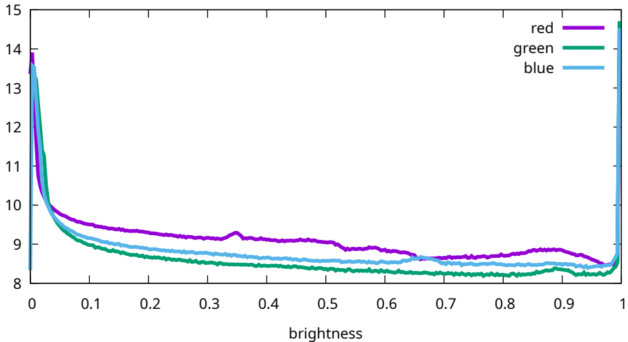
Flat histogram - Sony, ILCE-7M3, 80 ISO (7M30956)
