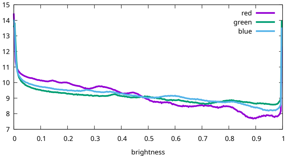
Flat histogram - Sony, ILCE-7M3, 4000 ISO (7M30973)
