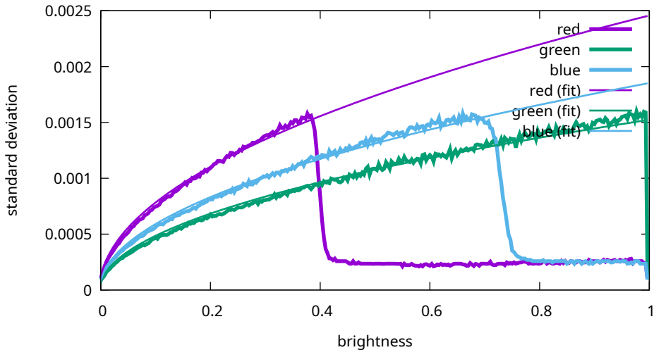
Noise levels - Sony, ILCE-7M3, 200 ISO (7M30960)
