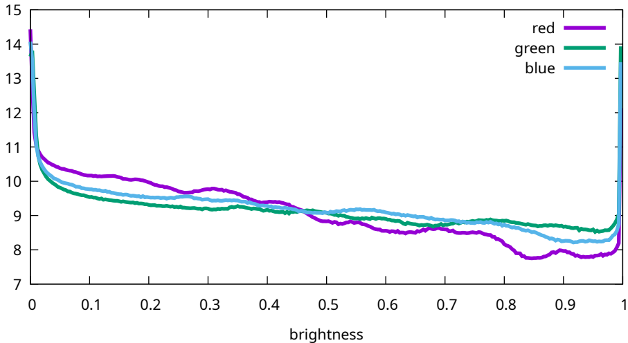
Flat histogram - Sony, ILCE-7M3, 6400 ISO (7M30975)
