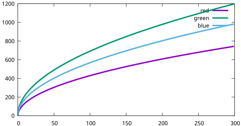
Conversion curves - Sony, ILCE-7M3, 250 ISO (7M30961)
