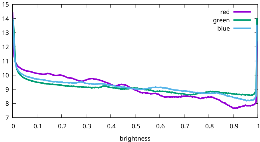
Flat histogram - Sony, ILCE-7M3, 3200 ISO (7M30972)
