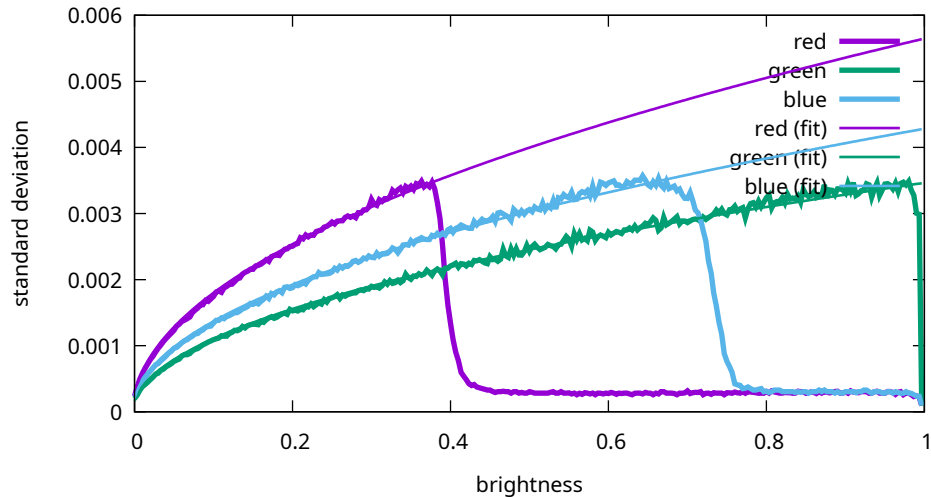
Noise levels - Sony, ILCE-7M3, 1250 ISO (7M30968)
