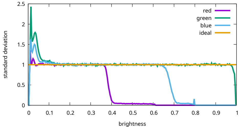
Flat noise levels - Sony, ILCE-7M3, 10000 ISO ( 7M30977 )
