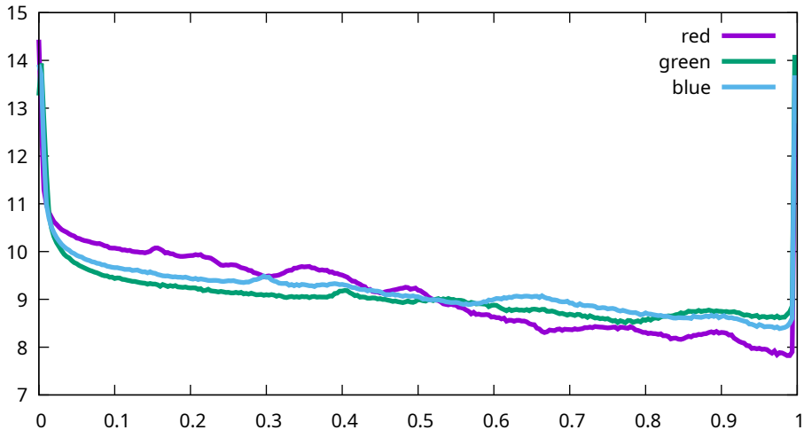
Histogram - Sony, ILCE-7M3, 1000 ISO (7M30967)
