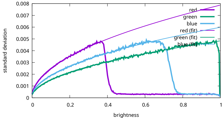
Noise levels - Sony, ILCE-7M3, 2500 ISO (7M30971)
