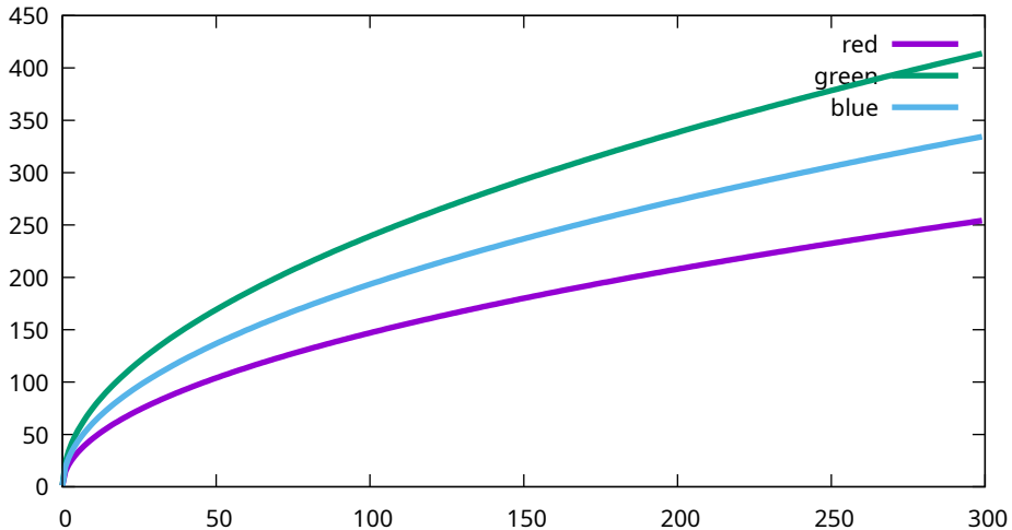
Conversion curves - Sony, ILCE-7M3, 2500 ISO (7M30971)
