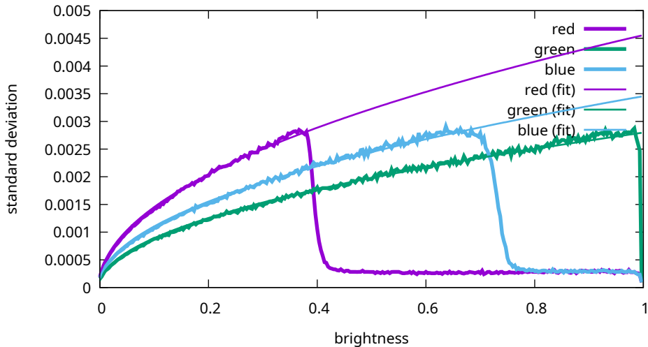
Noise levels - Sony, ILCE-7M3, 800 ISO (7M30966)
