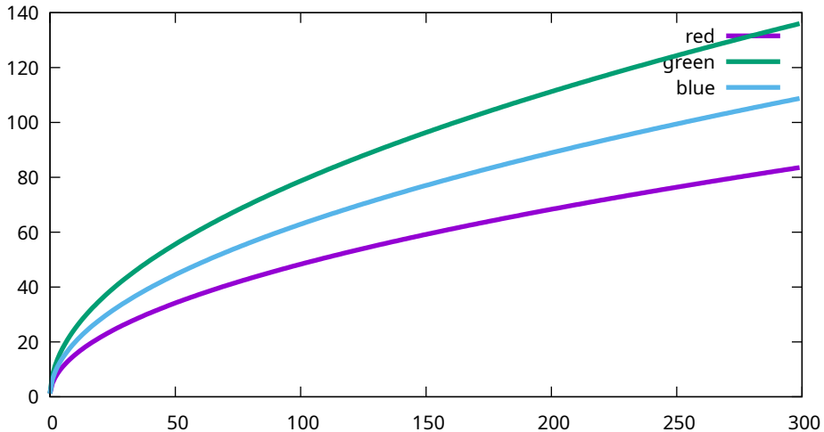
Conversion curves - Sony, ILCE-7M3, 25600 ISO (7M30981)
