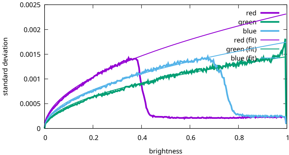
Noise levels - Sony, ILCE-7M3, 80 ISO (7M30956)
