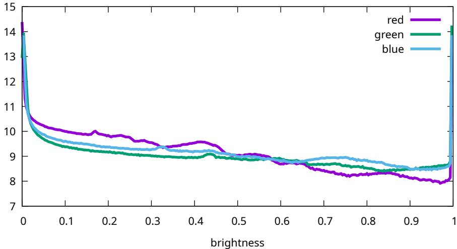
Flat histogram - Sony, ILCE-7M3, 200 ISO (7M30960)
