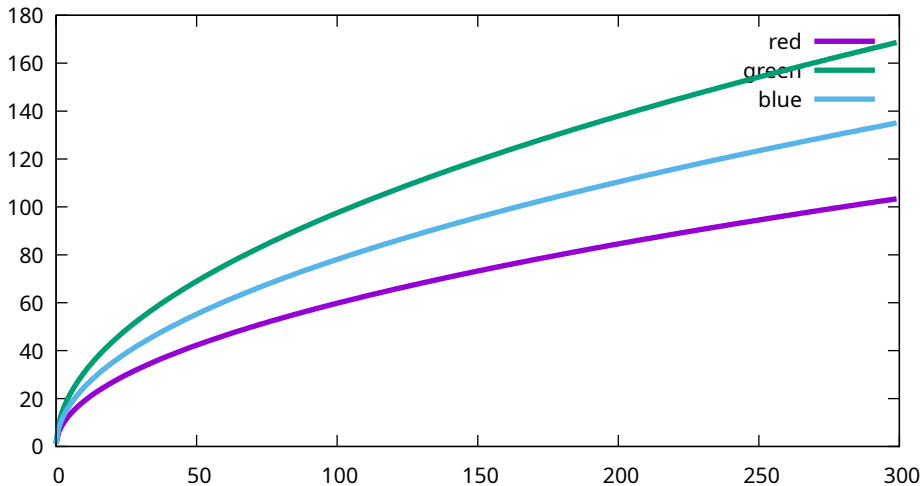
Conversion curves - Sony, ILCE-7M3, 16000 ISO (7M30979)
