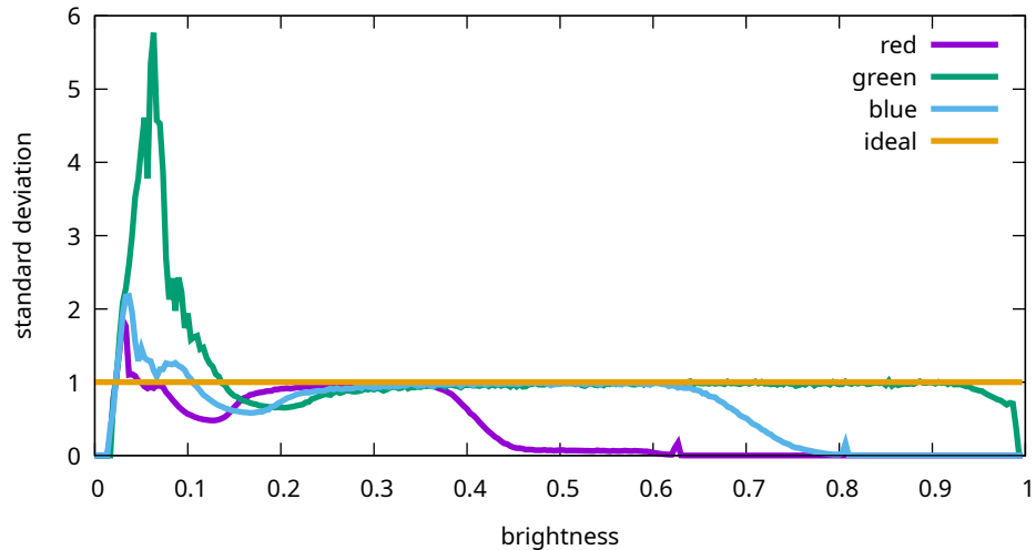
Flat noise levels - Sony, ILCE-7M3, 128000 ISO (7M30988)
