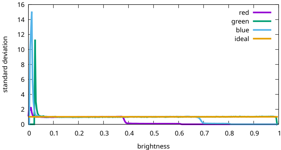
Flat noise levels - Sony, ILCE-7M3, 640 ISO (7M30965)
