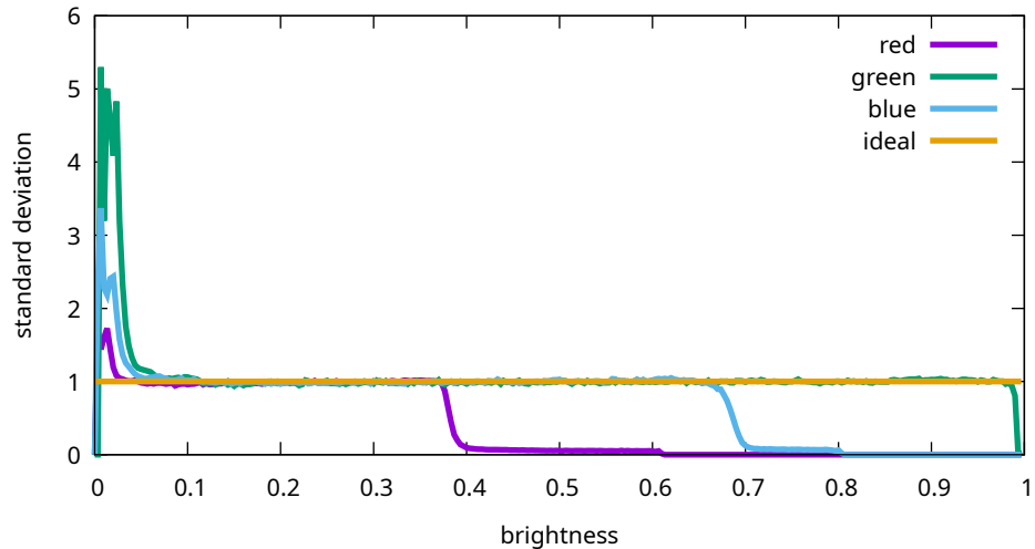
Flat noise levels - Sony, ILCE-7M3, 1600 ISO (7M30969)
