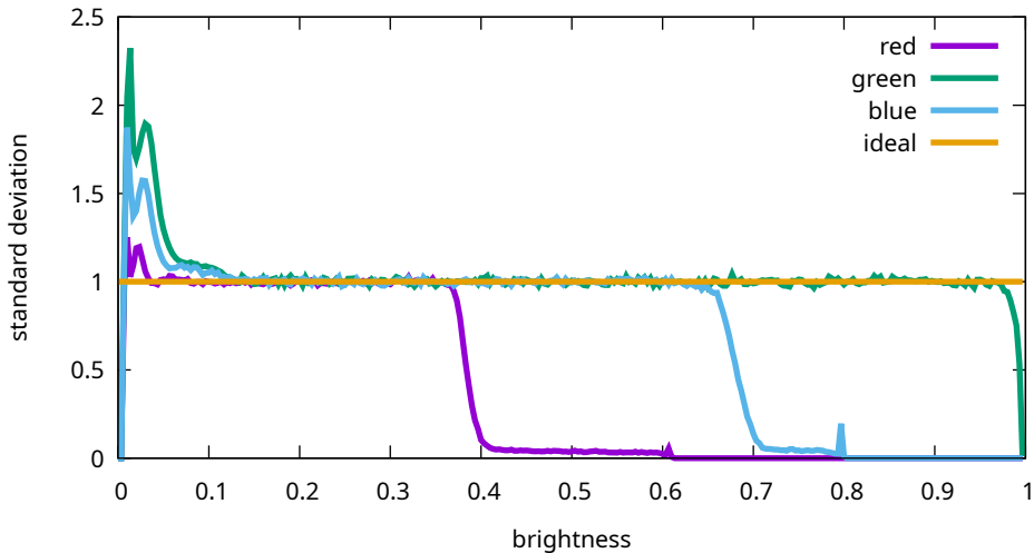
Flat noise levels - Sony, ILCE-7M3, 8000 ISO (7M30976)
