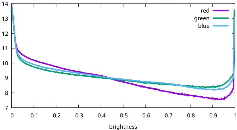
Flat histogram - Sony, ILCE-7M3, 102400 ISO (7M30986)
