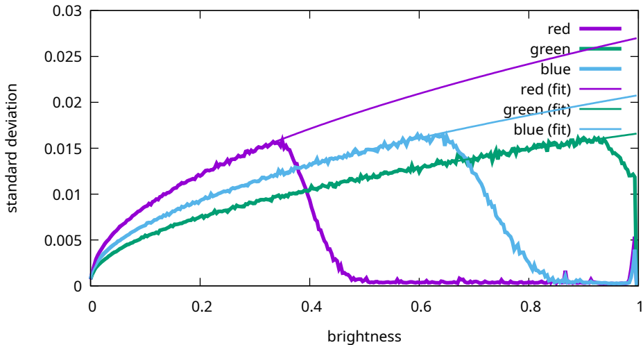
Noise levels - Sony, ILCE-7M3, 32000 ISO (7M30982)
