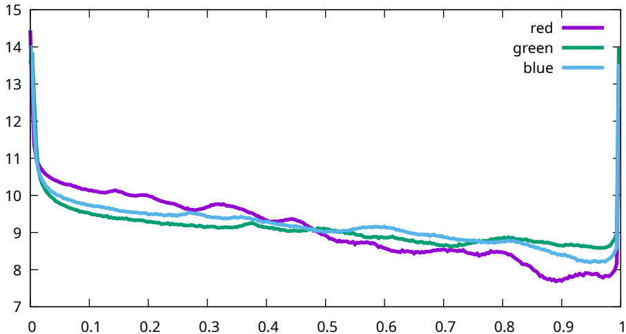
Histogram - Sony, ILCE-7M3, 4000 ISO (7M30973)
