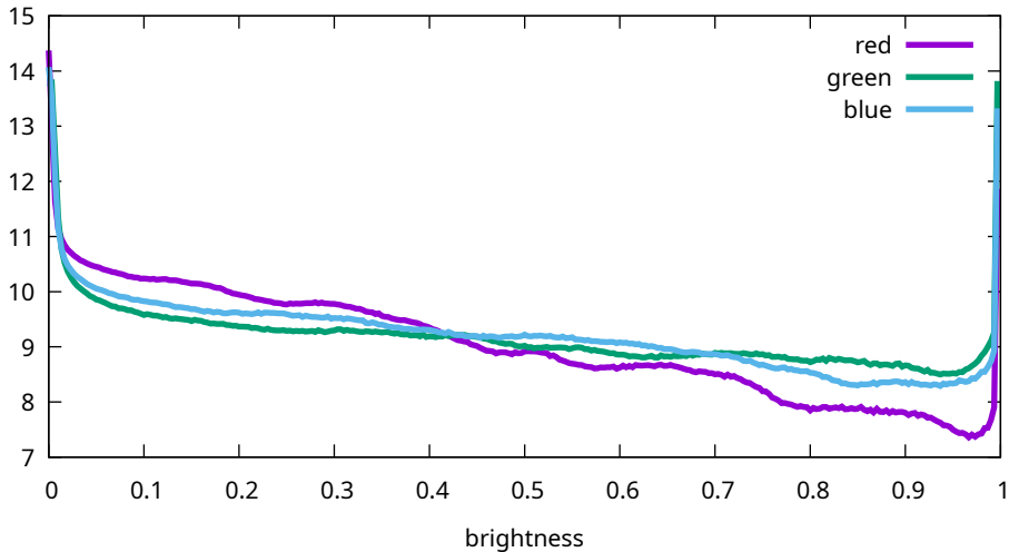
Flat histogram - Sony, ILCE-7M3, 12800 ISO (7M30978)
