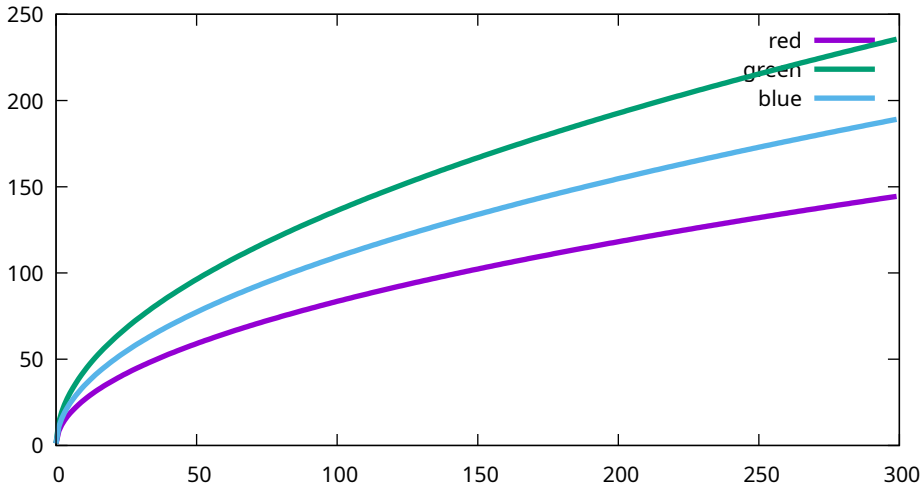
Conversion curves - Sony, ILCE-7M3, 8000 ISO (7M30976)
