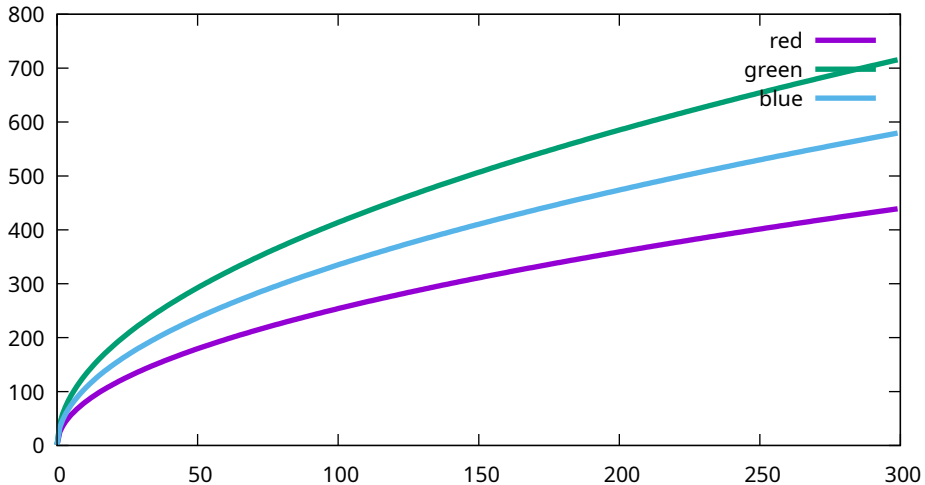
Conversion curves - Sony, ILCE-7M3, 800 ISO (7M30966)
