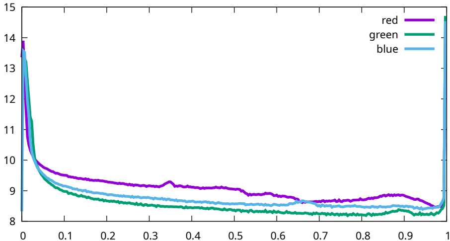
Histogram - Sony, ILCE-7M3, 80 ISO (7M30956)
