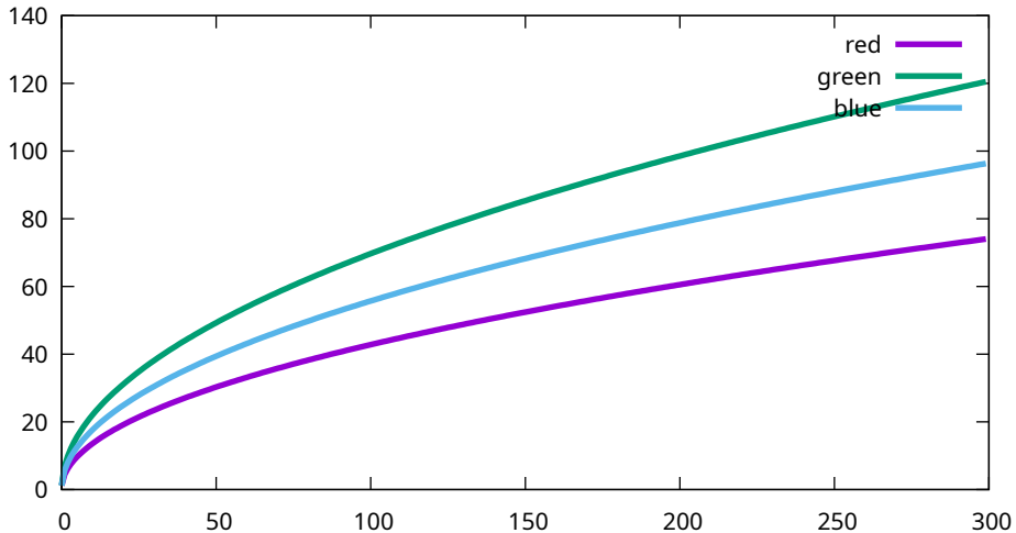
Conversion curves - Sony, ILCE-7M3, 32000 ISO (7M30982)
