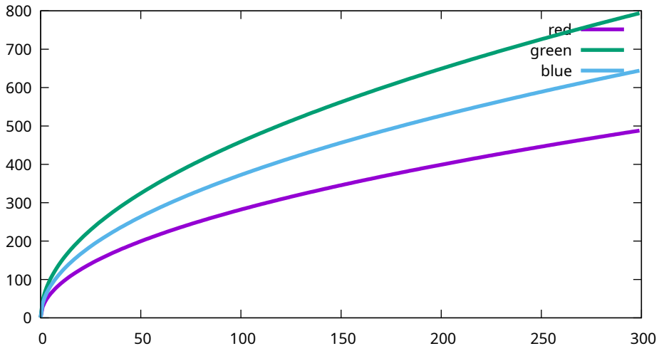
Conversion curves - Sony, ILCE-7M3, 640 ISO (7M30965)
