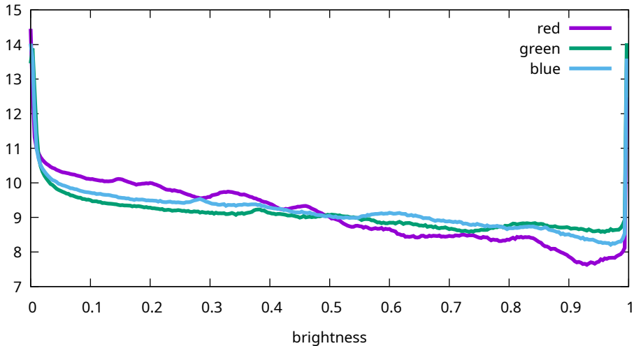
Flat histogram - Sony, ILCE-7M3, 2500 ISO (7M30971)
