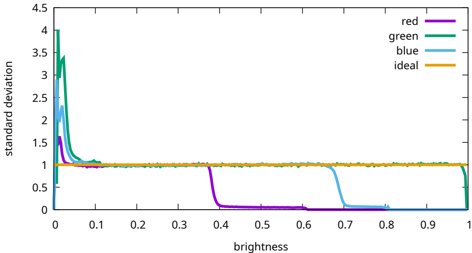
Flat noise levels - Sony, ILCE-7M3, 2000 ISO (7M30970)
