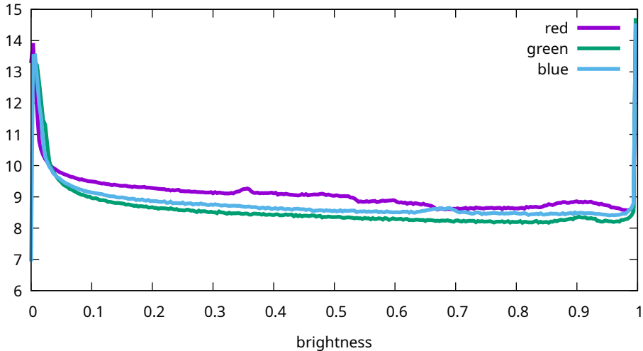
Flat histogram - Sony, ILCE-7M3, 64 ISO (7M30955)
