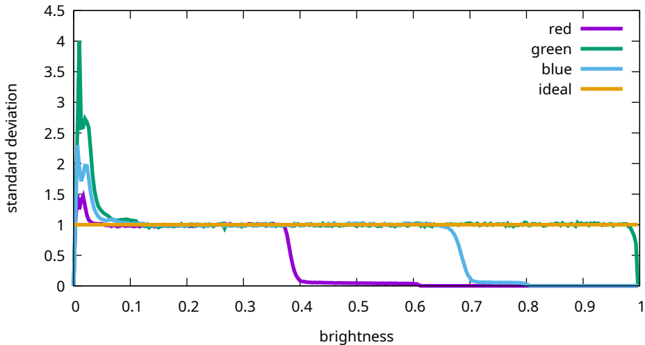
Flat noise levels - Sony, ILCE-7M3, 3200 ISO (7M30972)
