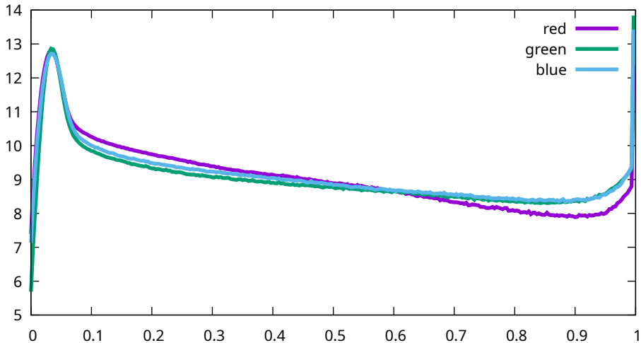
Histogram - Sony, ILCE-7M3, 160000 ISO (7M30989)
