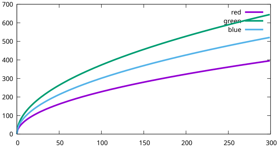
Conversion curves - Sony, ILCE-7M3, 1000 ISO (7M30967)
