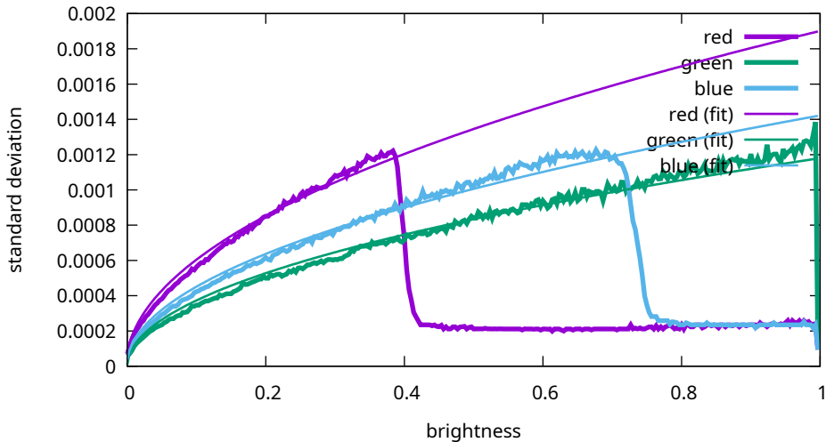
Noise levels - Sony, ILCE-7M3, 100 ISO (7M30957)
