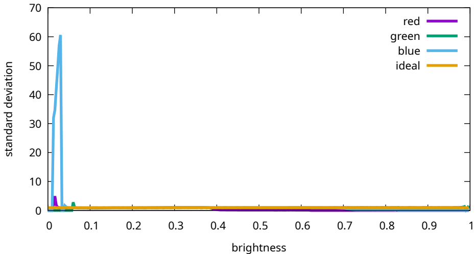
Flat noise levels - Sony, ILCE-7M3, 80 ISO (7M30956)
