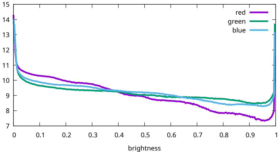
Flat histogram - Sony, ILCE-7M3, 20000 ISO (7M30980)
