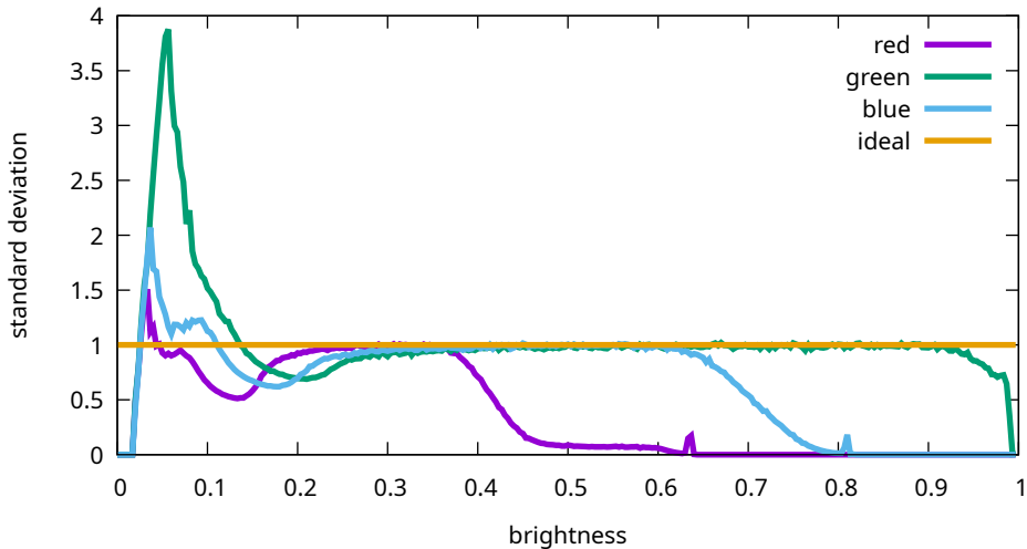
Flat noise levels - Sony, ILCE-7M3, 160000 ISO (7M30989)
