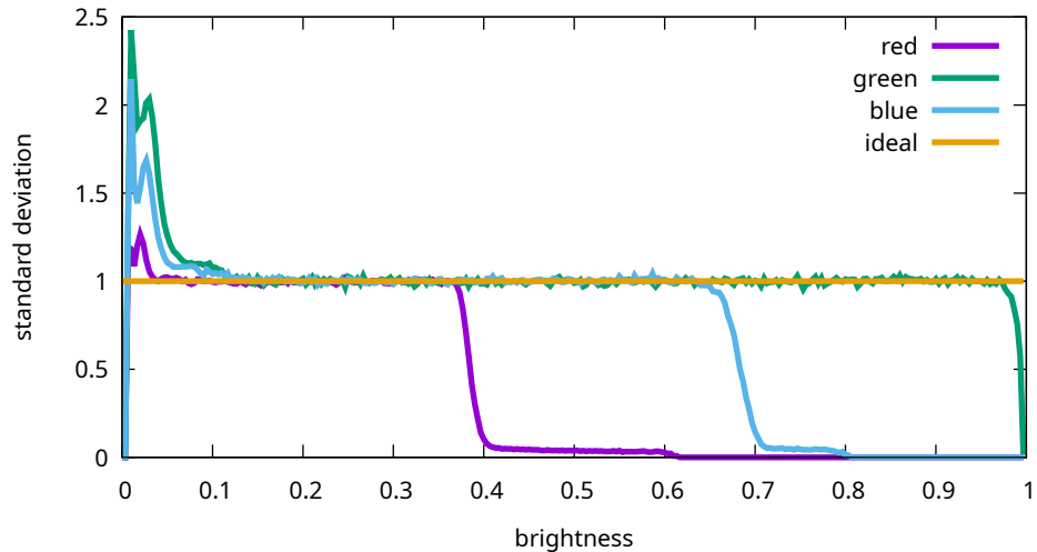
Flat noise levels - Sony, ILCE-7M3, 6400 ISO (7M30975)
