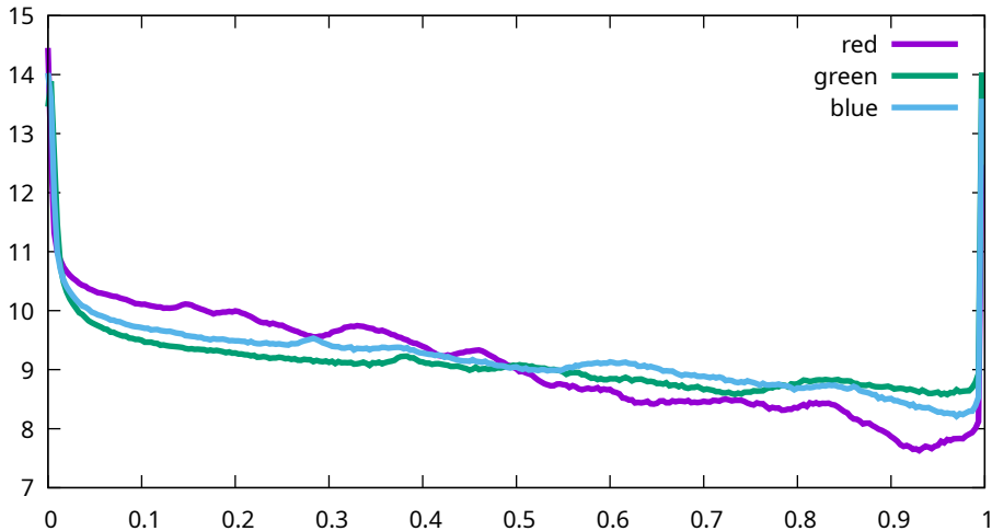
Histogram - Sony, ILCE-7M3, 2500 ISO (7M30971)
