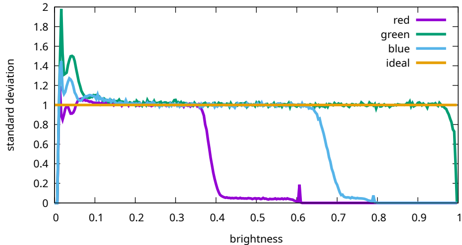
Flat noise levels - Sony, ILCE-7M3, 20000 ISO ( 7M30980 )
