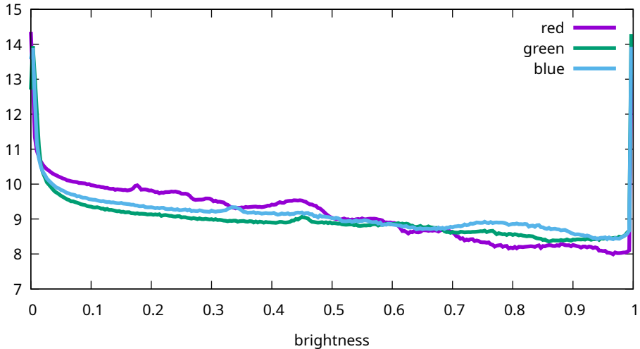
Flat histogram - Sony, ILCE-7M3, 100 ISO (7M30957)
