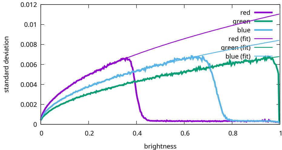
Noise levels - Sony, ILCE-7M3, 5000 ISO (7M30974)
