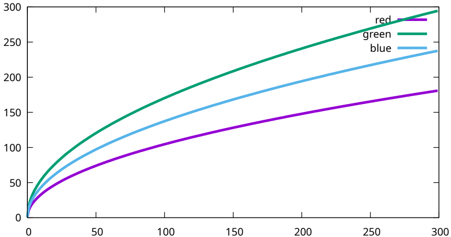
Conversion curves - Sony, ILCE-7M3, 5000 ISO (7M30974)
