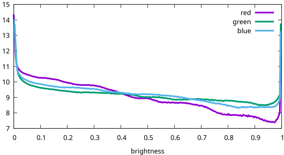
Flat histogram - Sony, ILCE-7M3, 16000 ISO (7M30979)
