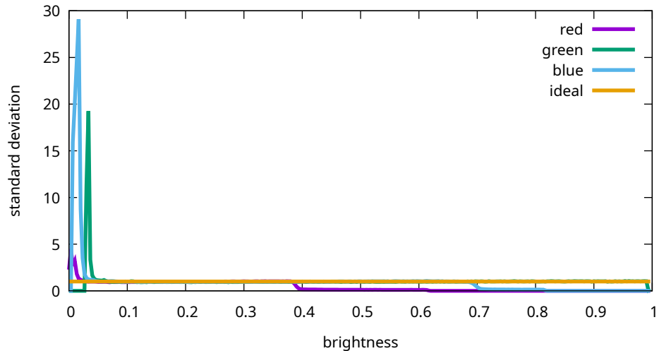
Flat noise levels - Sony, ILCE-7M3, 250 ISO ( 7 M30961)
