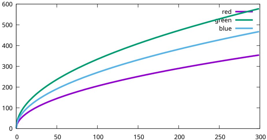
Conversion curves - Sony, ILCE-7M3, 1250 ISO (7M30968)
