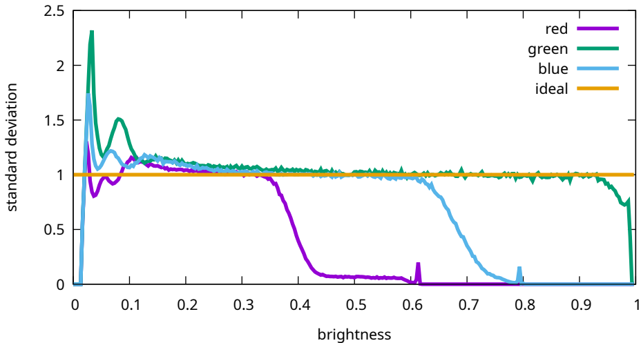
Flat noise levels - Sony, ILCE-7M3, 102400 ISO (7M30986)
