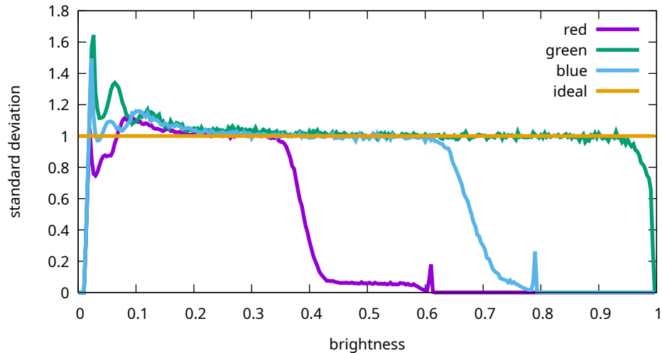
Flat noise levels - Sony, ILCE-7M3, 51200 ISO ( 7M30984 )
