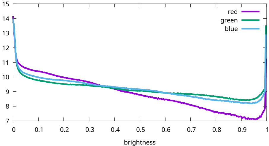
Flat histogram - Sony, ILCE-7M3, 40000 ISO (7M30983)
