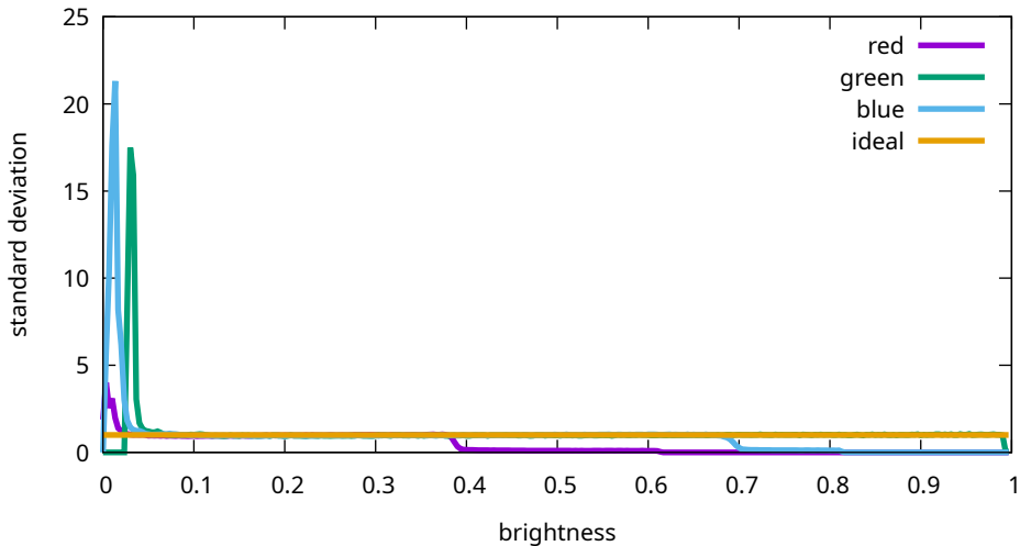
Flat noise levels - Sony, ILCE-7M3, 320 ISO ( 7 M30962)
