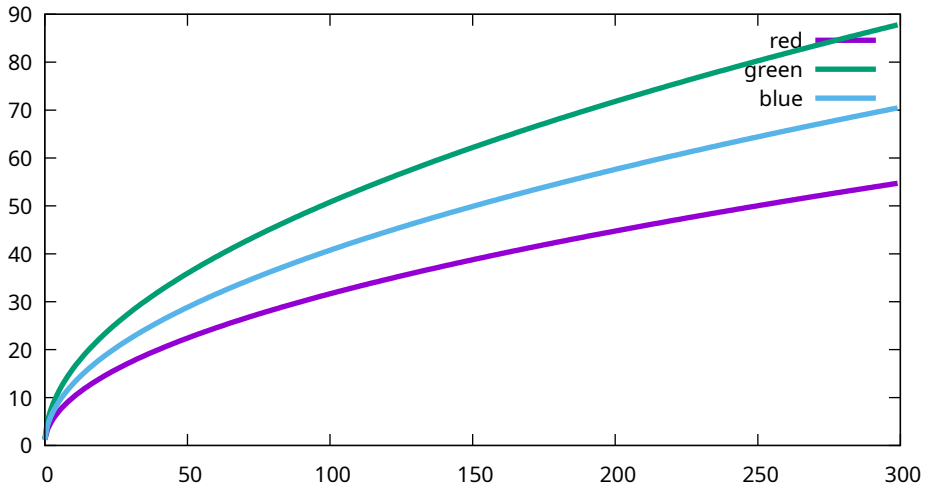
Conversion curves - Sony, ILCE-7M3, 102400 ISO (7M30987)
