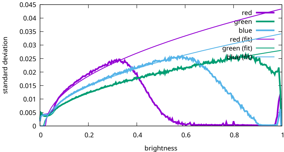
Noise levels - Sony, ILCE-7M3, 160000 ISO (7M30989)
