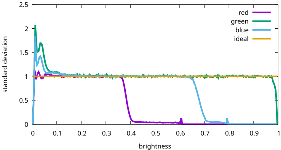
Flat noise levels - Sony, ILCE-7M3, 12800 ISO ( 7M30978 )
