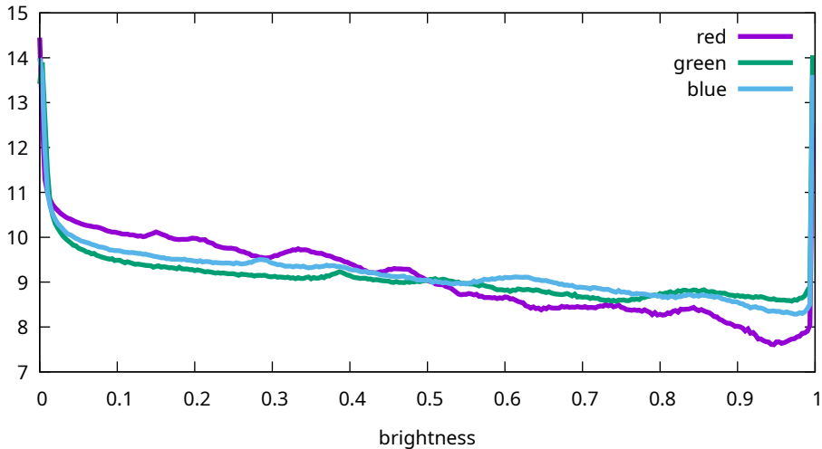
Flat histogram - Sony, ILCE-7M3, 2000 ISO (7M30970)
