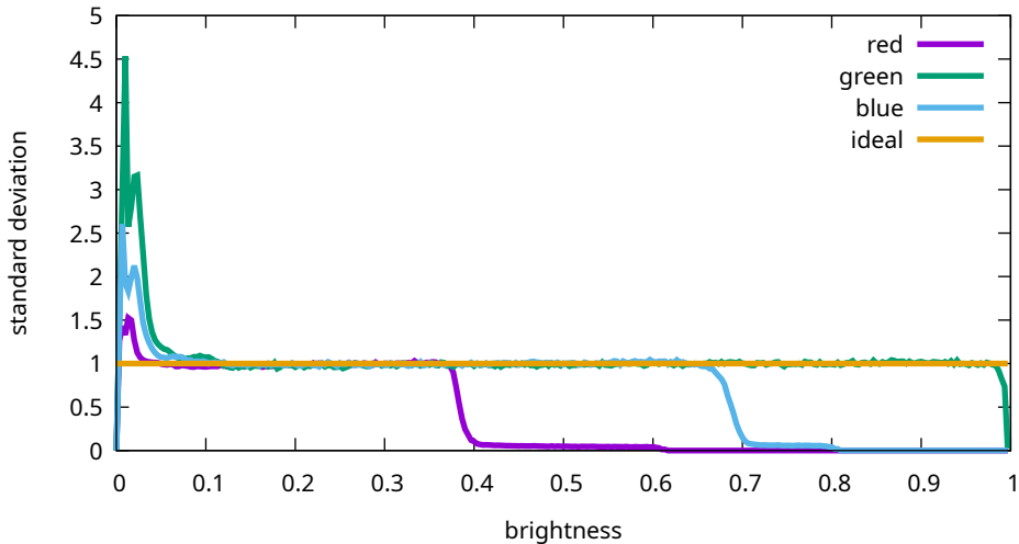
Flat noise levels - Sony, ILCE-7M3, 2500 ISO (7M30971)
