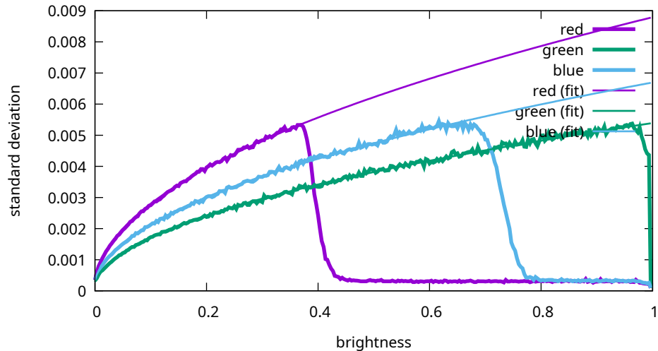
Noise levels - Sony, ILCE-7M3, 3200 ISO (7M30972)
