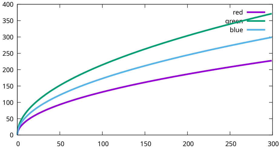
Conversion curves - Sony, ILCE-7M3, 3200 ISO (7M30972)
