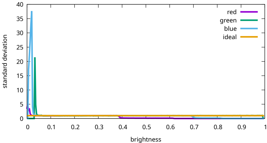
Flat noise levels - Sony, ILCE-7M3, 200 ISO ( 7 M30960)
