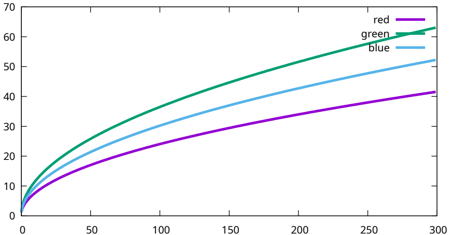
Conversion curves - Sony, ILCE-7M3, 204800 ISO ( 7 M30990)
