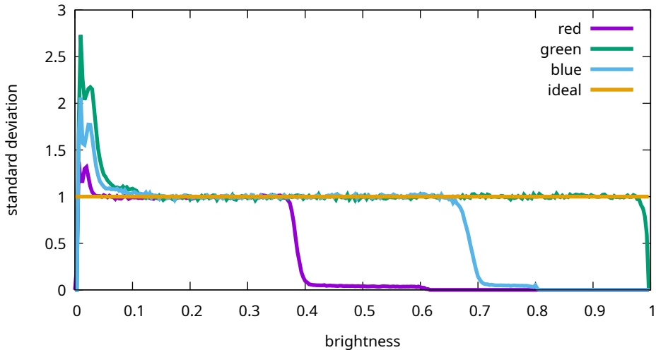
Flat noise levels - Sony, ILCE-7M3, 5000 ISO (7M30974)
