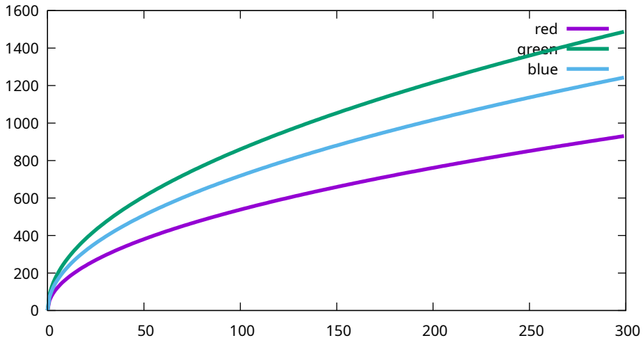
Conversion curves - Sony, ILCE-7M3, 64 ISO (7M30955)
