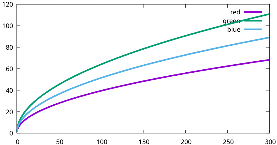
Conversion curves - Sony, ILCE-7M3, 64000 ISO (7M30985)
