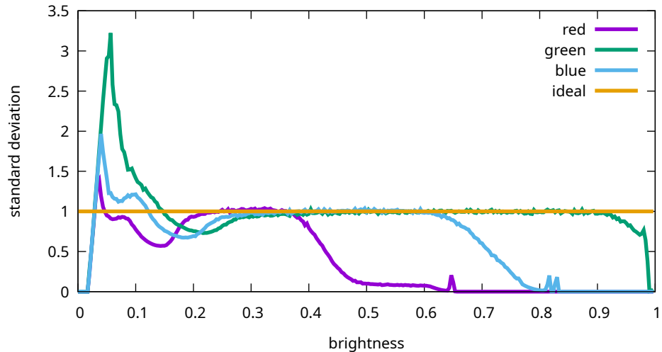
Flat noise levels - Sony, ILCE-7M3, 204800 ISO (7M30990)
