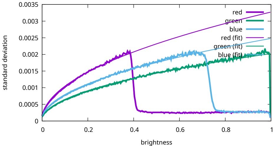
Noise levels - Sony, ILCE-7M3, 400 ISO (7M30963)
