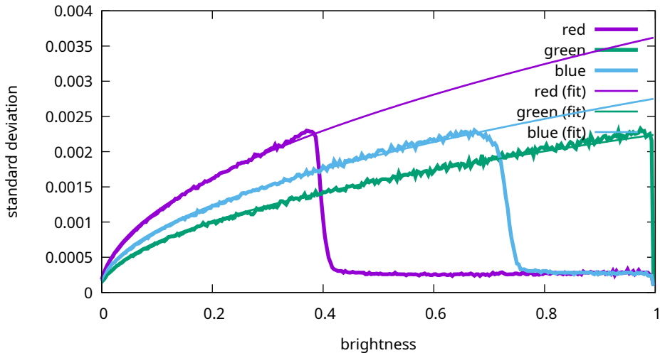
Noise levels - Sony, ILCE-7M3, 500 ISO (7M30964)
